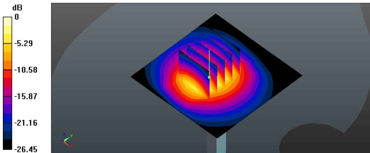
0 dB = 23.8 W/kg
