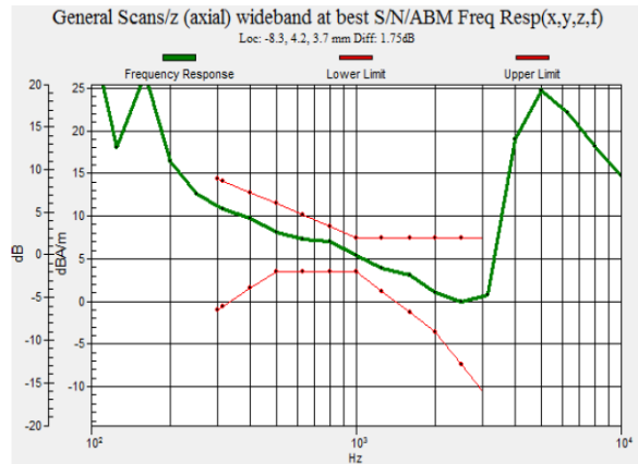
Fig 7.2 GSM1900 Ch661
