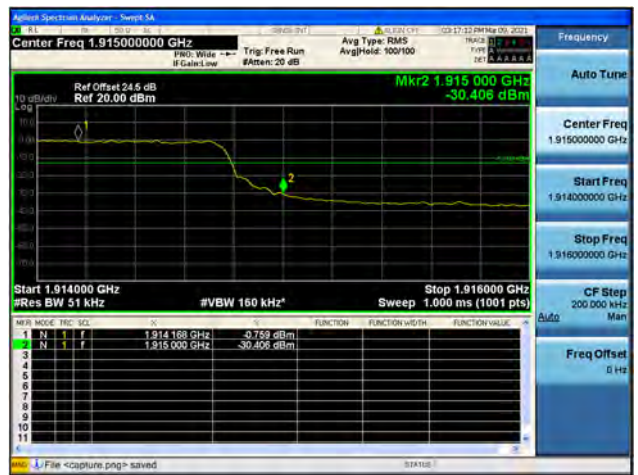
Band25 / 5MHz / High CH / QPSK / FULL RB
