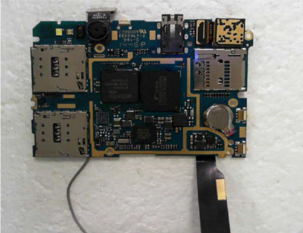
Mainboard Rear
