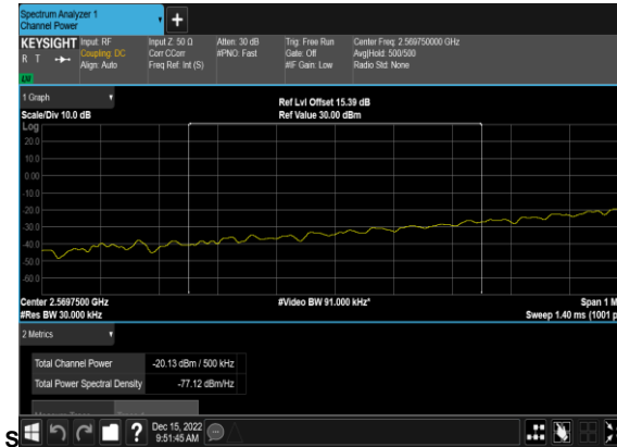
N38(25M)_DFT-s-OFDM_QPSK_Edge_1RB_Left_Low_CH_CHP_PAS
