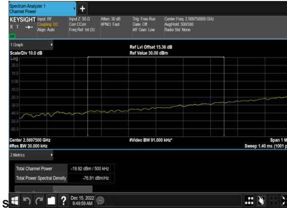
N38(25M)_DFT-s-OFDM_BPSK_Edge_1RB_Left_Low_CH_CHP_PAS
