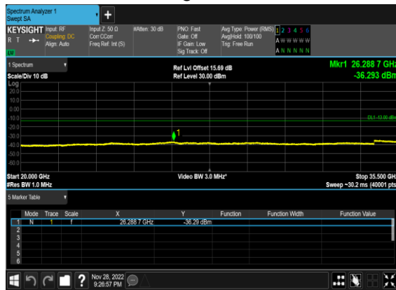
N78(20M)_DFT-s-OFDM_BPSK_Edge_1RB_Left_Mid_CH
