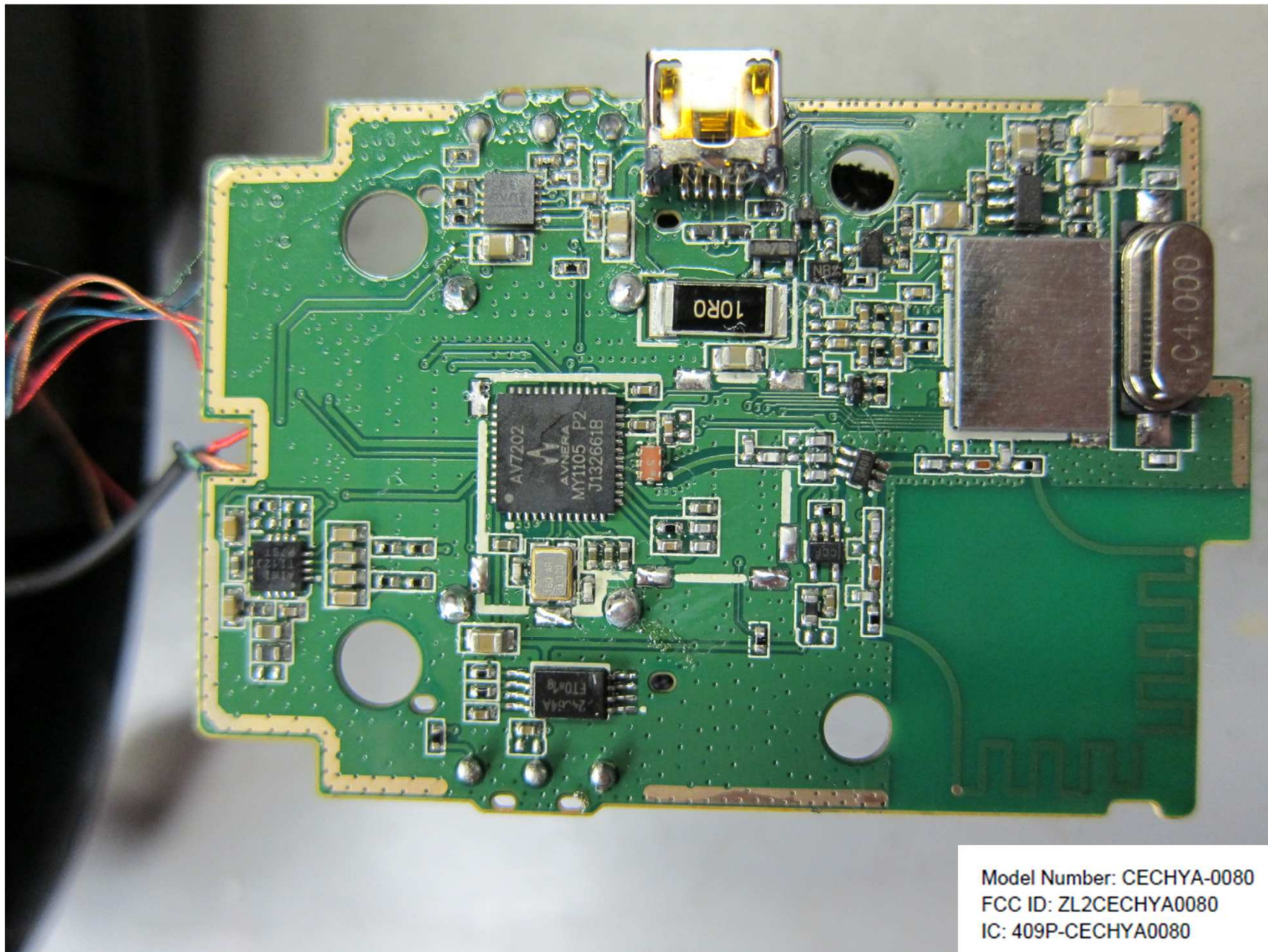
Internal photograph of Wireless Headset (Shield Removed)
