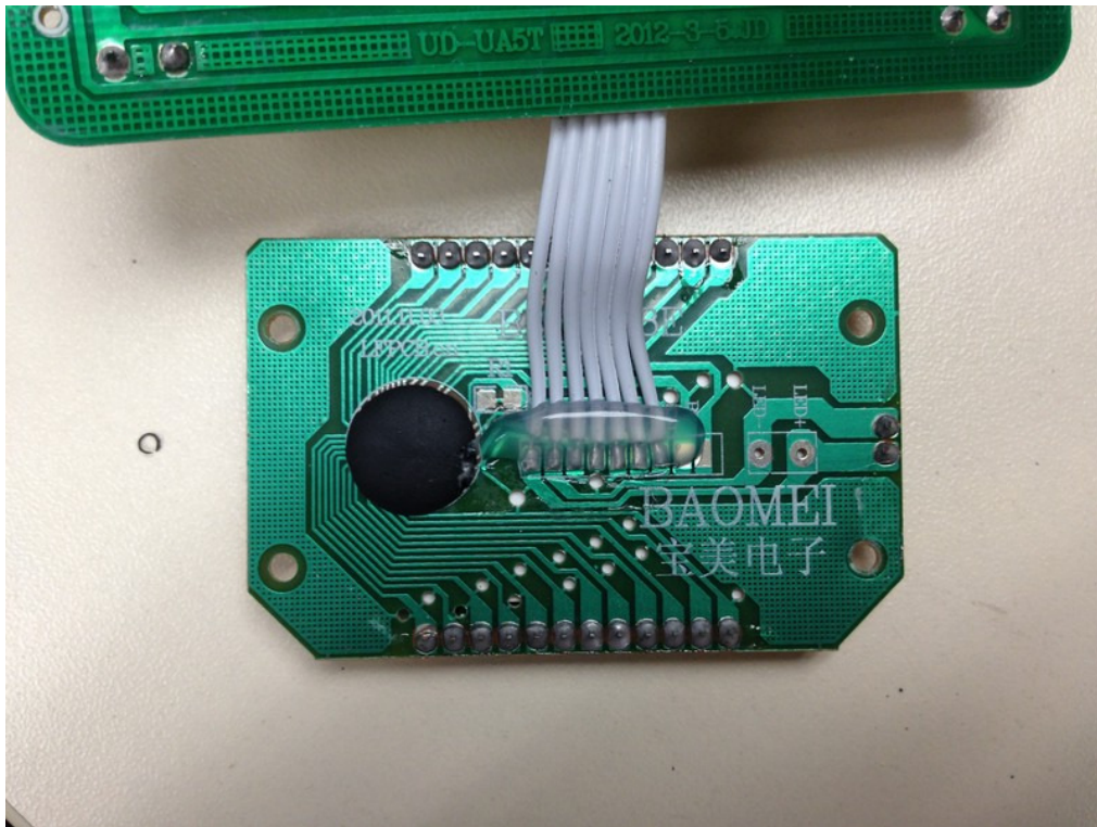
Internal View (Transmitter)
