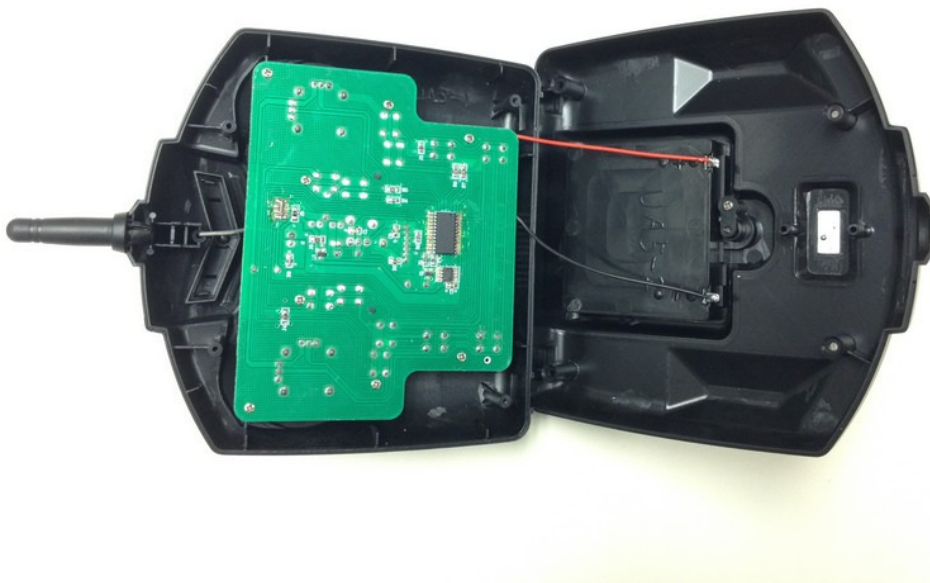
Internal View (Transmitter)
