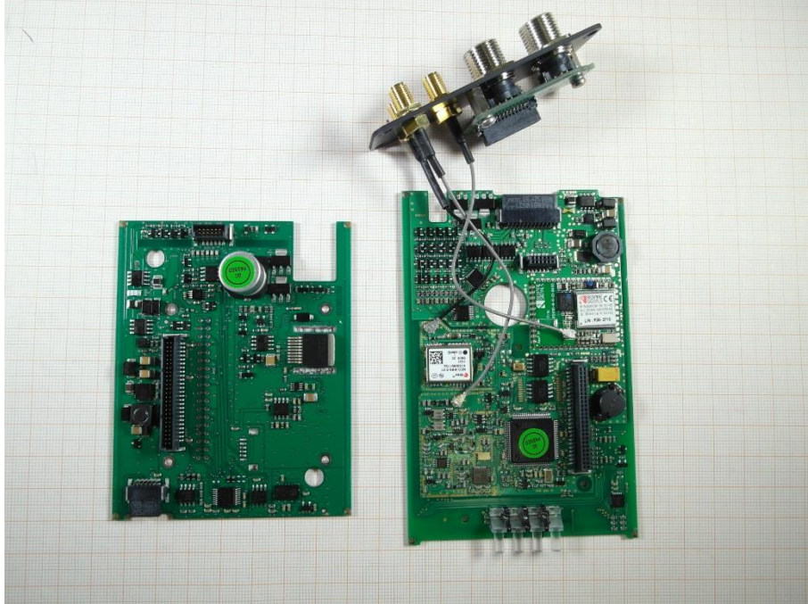
Photo 3: PCBs detached
