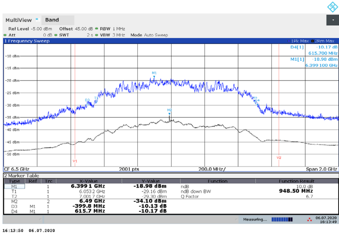
Plot 1: 10 dB down
