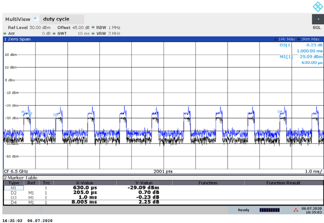
Plot 2: Duty Cycle, test mode
