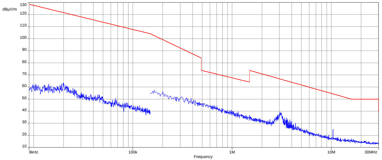
Plot 6: 15.209, TX 9 kHz – 30 MHz
