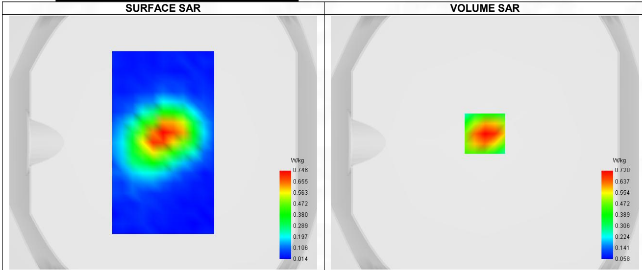
Maximum location: X=0.00, Y=7.00 ; SAR Peak: 1.10 W/kg
