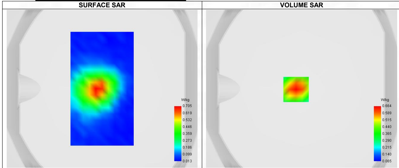
Maximum location: X=-7.00, Y=-1.00 ; SAR Peak: 0.95 W/kg
