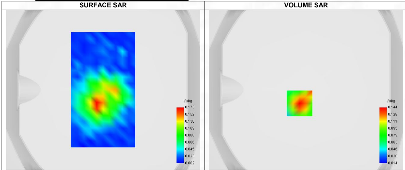
Maximum location: X=-8.00, Y=-17.00 ; SAR Peak: 0.21 W/kg
