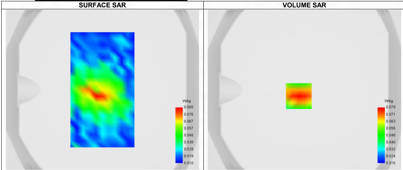
Maximum location: X=-7.00, Y=-8.00 ; SAR Peak: 0.12 W/kg
