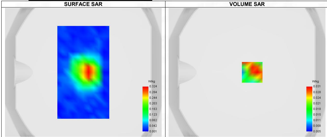
Maximum location: X=8.00, Y=0.00 ; SAR Peak: 0.06 W/kg
