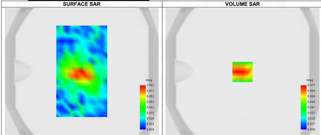
Maximum location: X=0.00, Y=-1.00 ; SAR Peak: 0.13 W/kg
