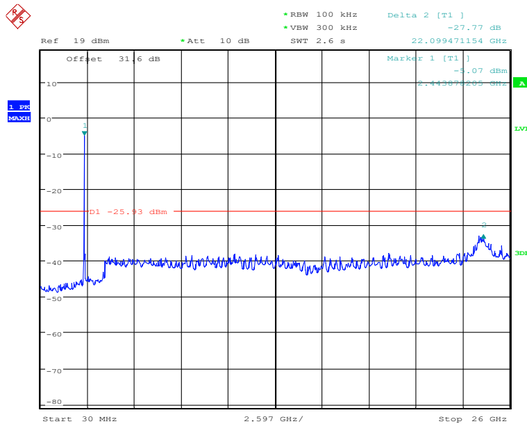
Fig.59 Conducted spurious emission: Ch11,11n(40M),2462MHz
