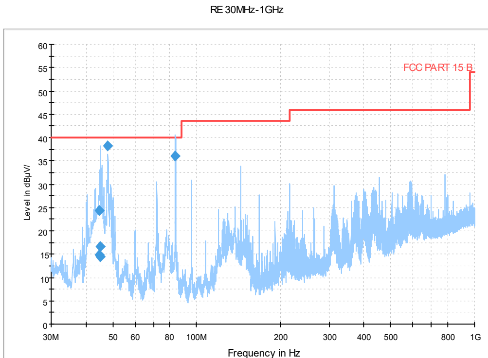
Fig.61 Radiated emission: Ch1, 30MHz-1GHz
