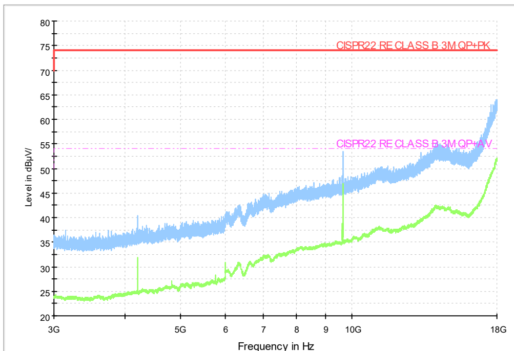
Fig.63 Radiated emission: Ch1, 3GHz-18GHz
