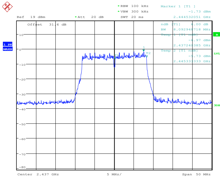
Fig.21 6dB Bandwidth: Ch6,11b
