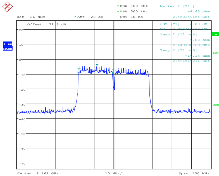
Fig.27 6dB Bandwidth: Ch11,11n
