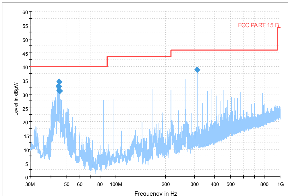
Fig.64 Radiated emission:Ch6, 30MHz-1GHz
