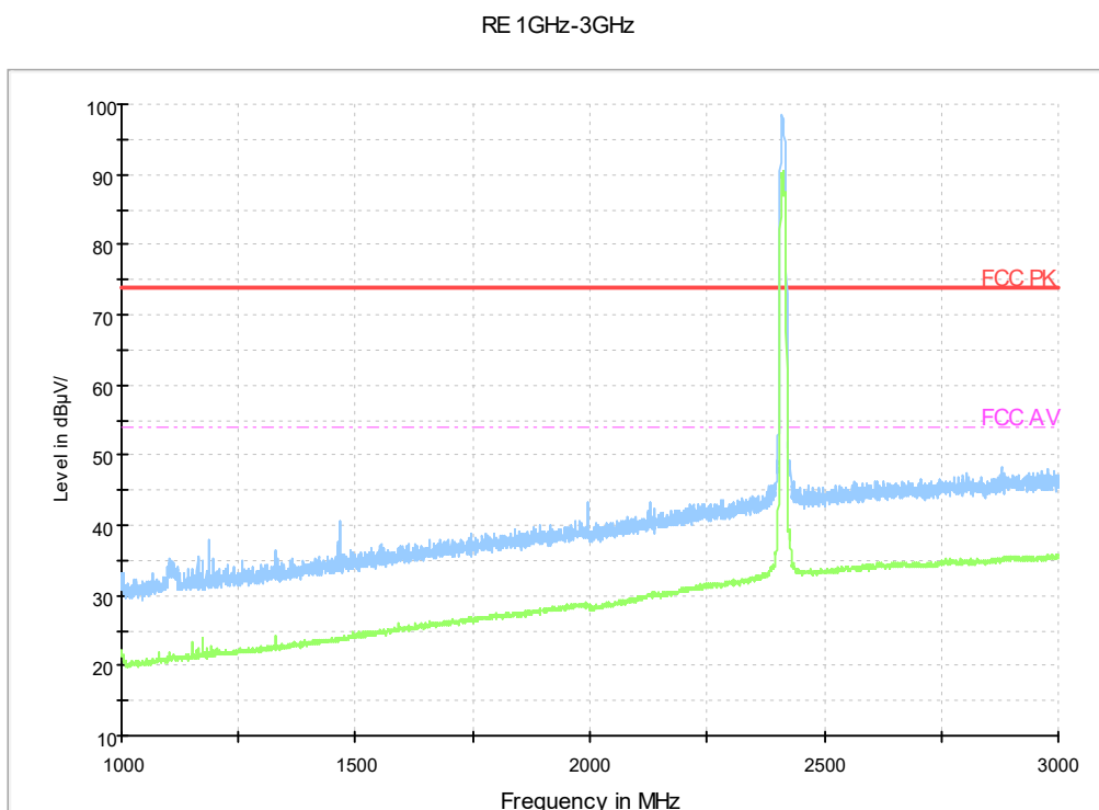
Fig.62 Radiated emission: Ch1, 1GHz-3GHz
