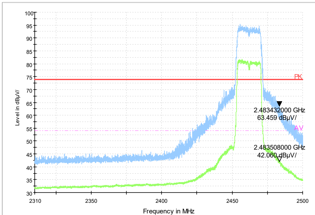
Fig.32 Frequency Band Edge: Ch11,11g
