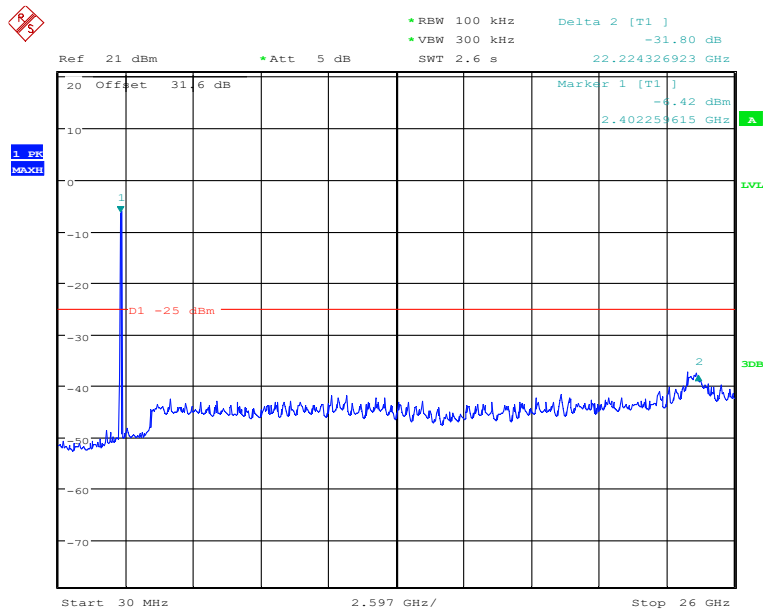
Fig.55 Conducted spurious emission: Ch1,1n(40M),2422MHz
