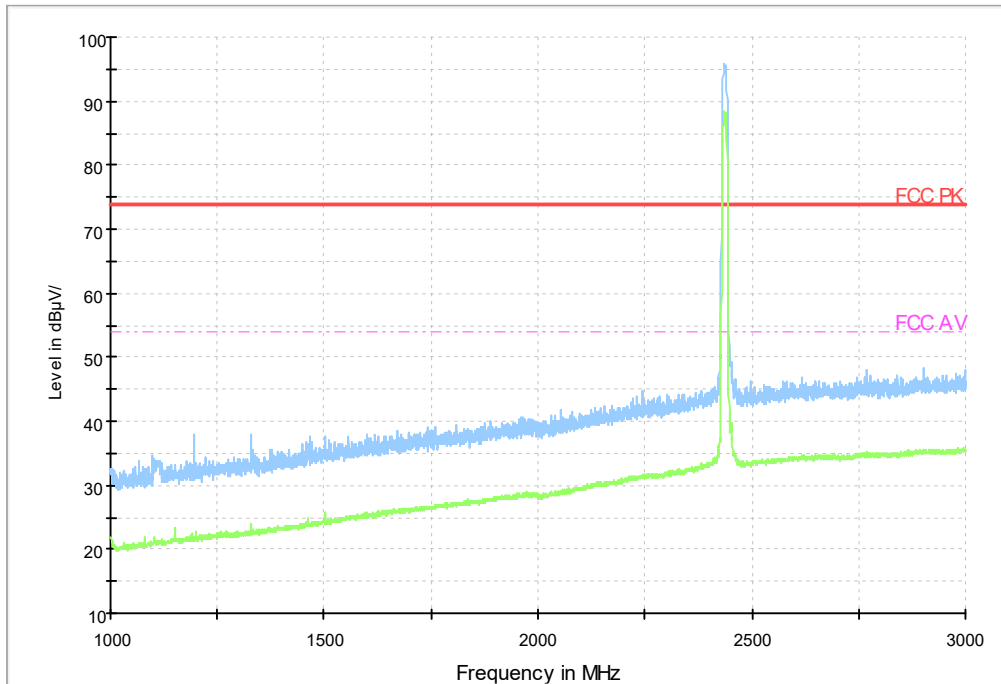
Fig.65 Radiated emission: Ch6, 1GHz-3GHz
