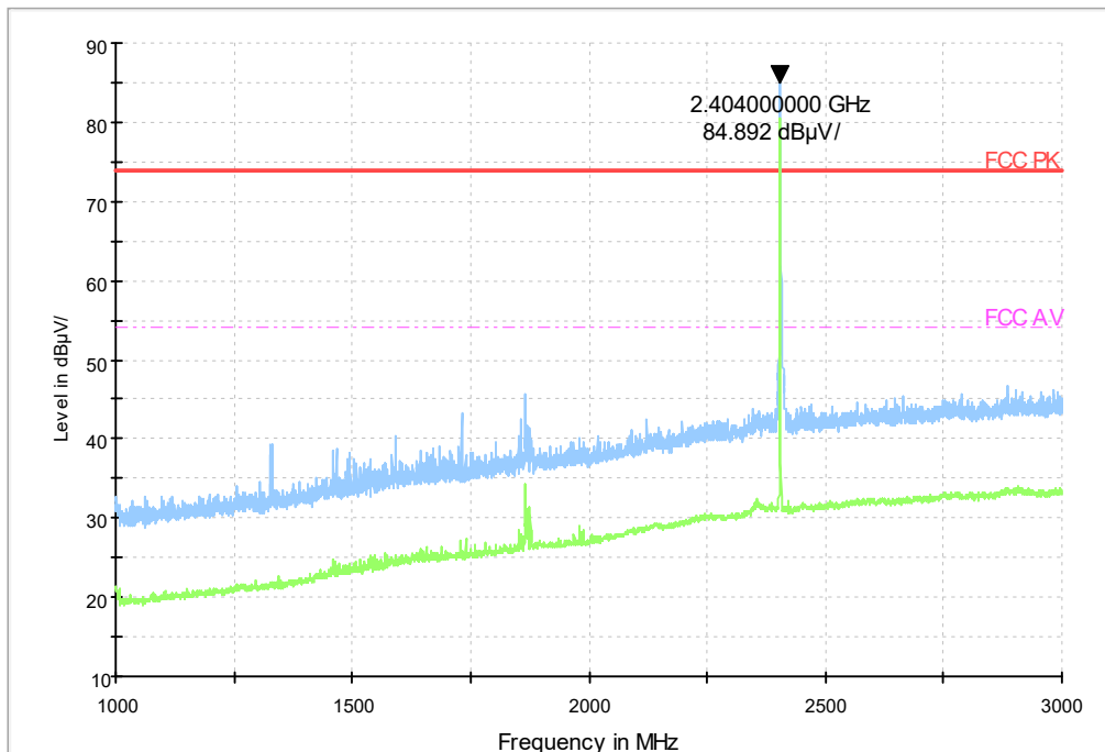
Fig.19 Radiated emission: Ch1, 1GHz-3GHz
