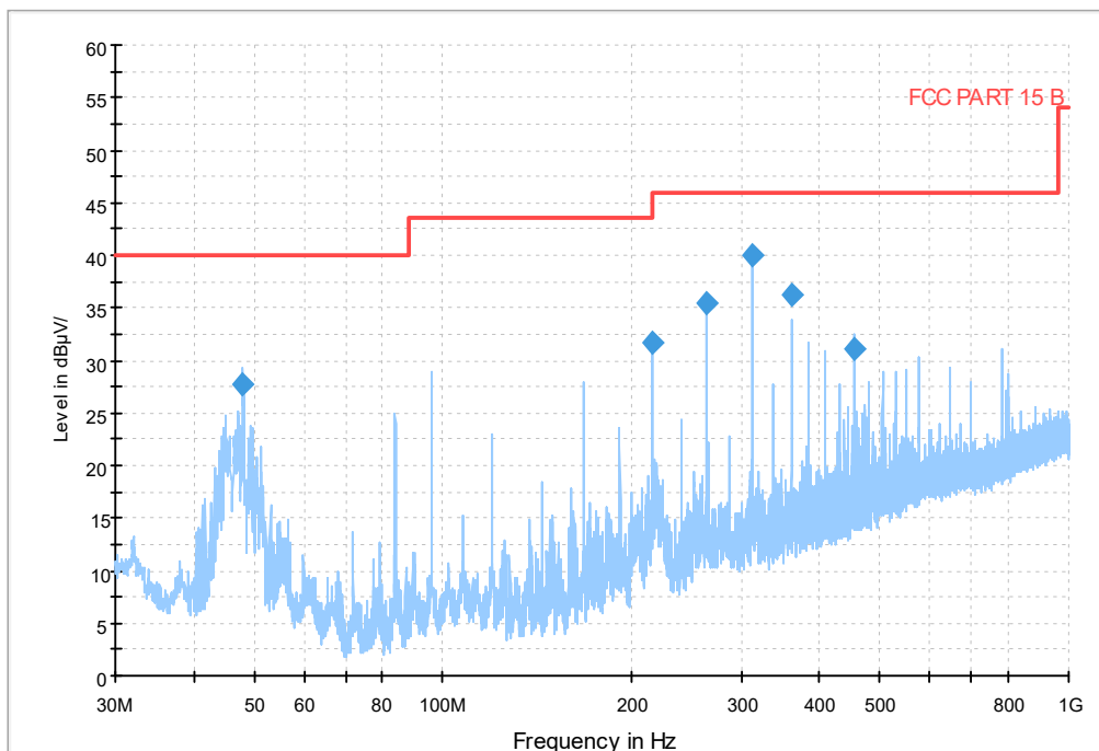
Fig.21 Radiated emission:Ch20, 30MHz-1GHz
