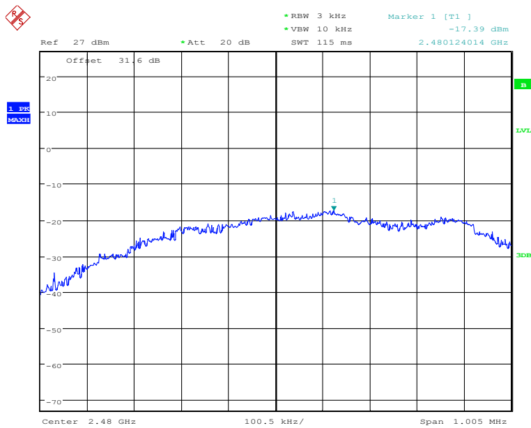
Fig.2 Power spectral density: CH19 PSD/3KHz
