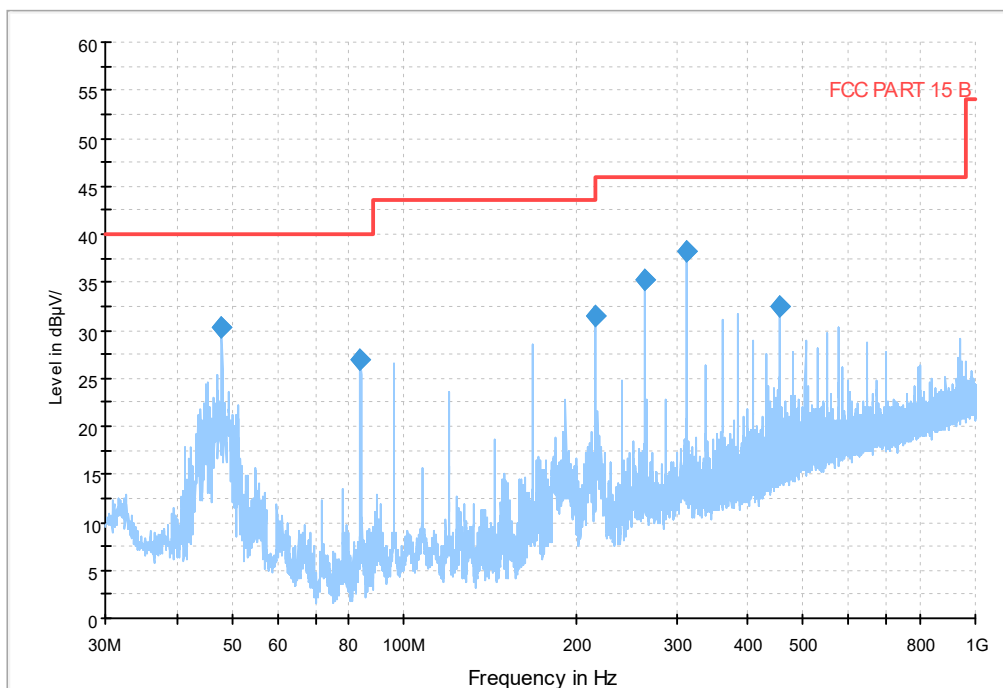
Fig.18 Radiated emission: Ch1, 30MHz-1GHz
