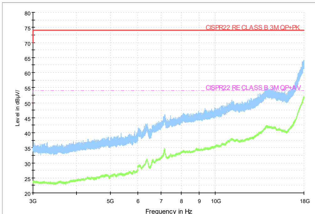
Fig.20 Radiated emission: Ch1, 3GHz-18GHz
