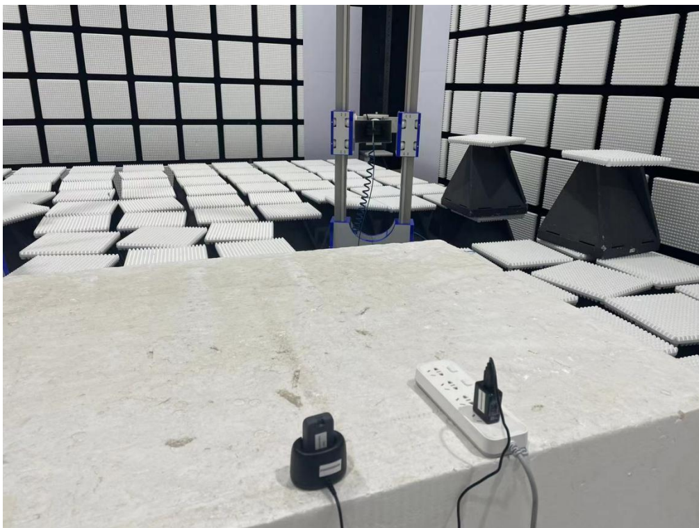
Pic2.Radiatedemissions(1GHz-18GHz)
