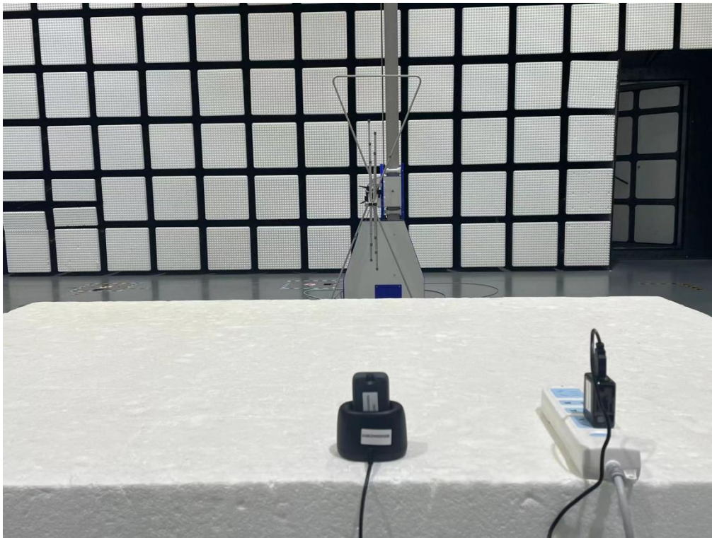
Pic1.Radiatedemissions(30MHz-1GHz)
