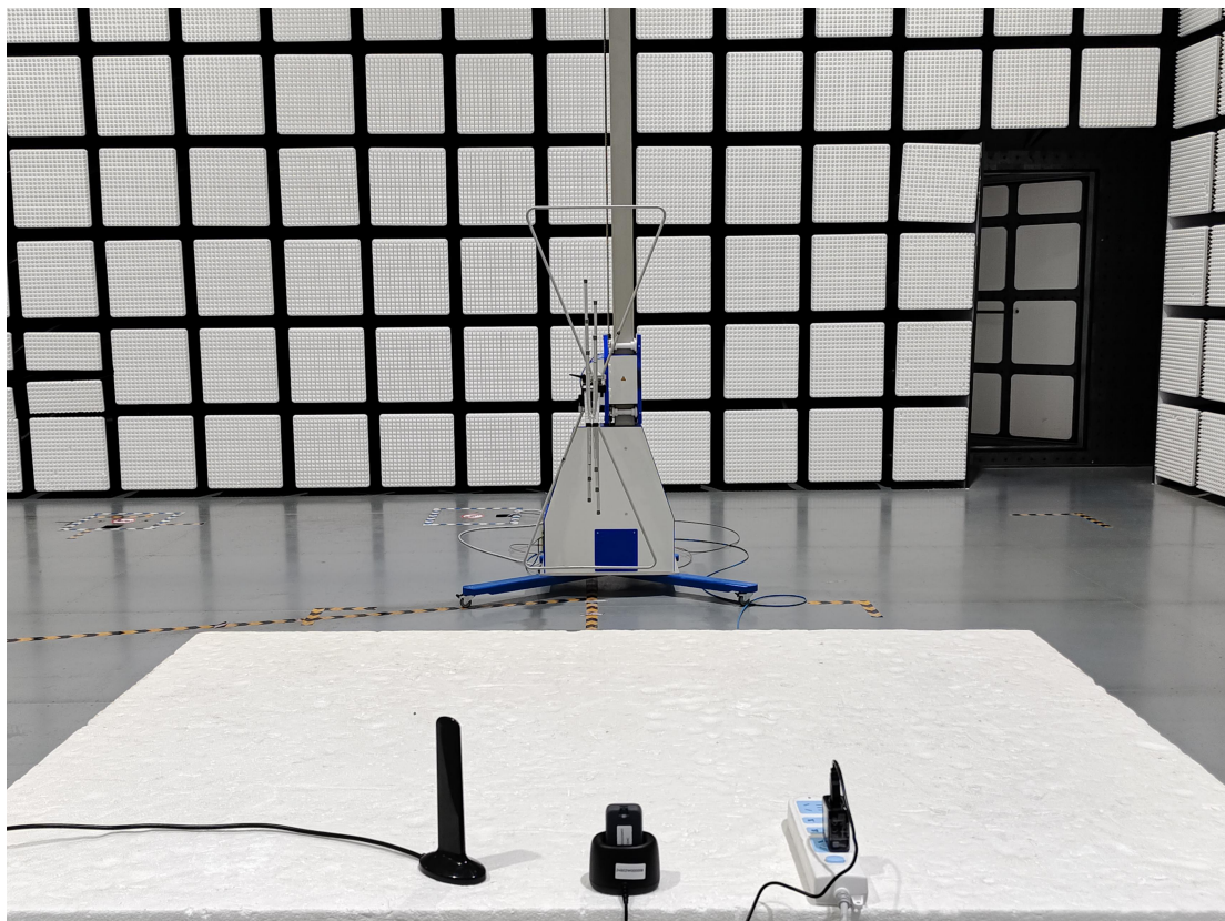
Pic4.RSE(30MHz-1GHz)
