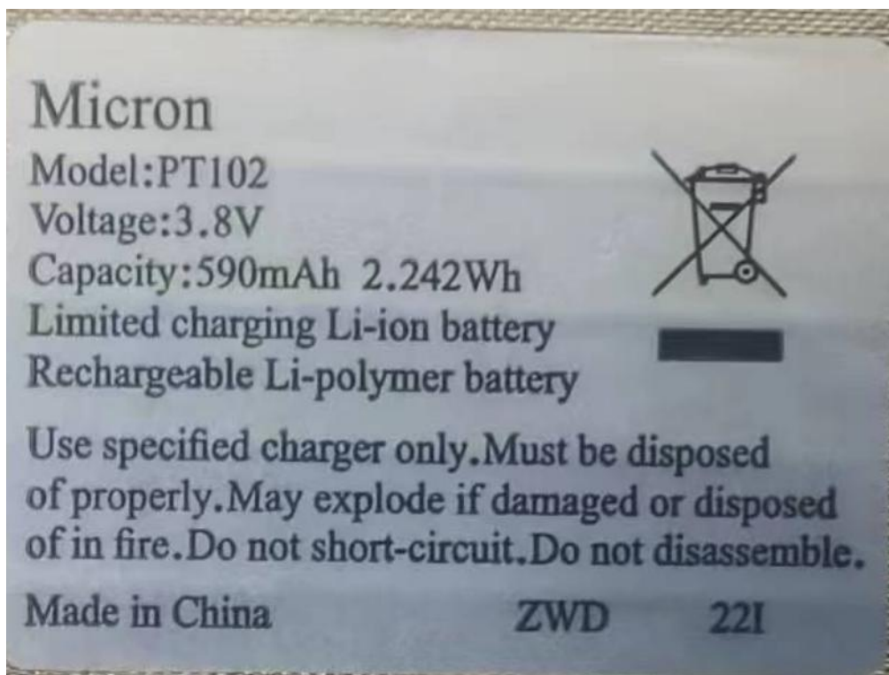
Battery label
