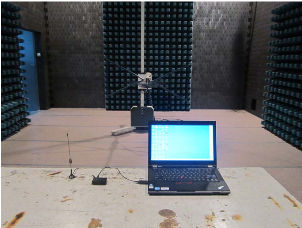
Radiated Emission test photo
