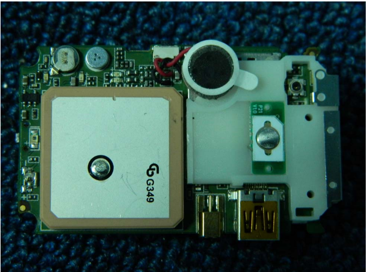
Fig.4 Mainboard (obverse)
