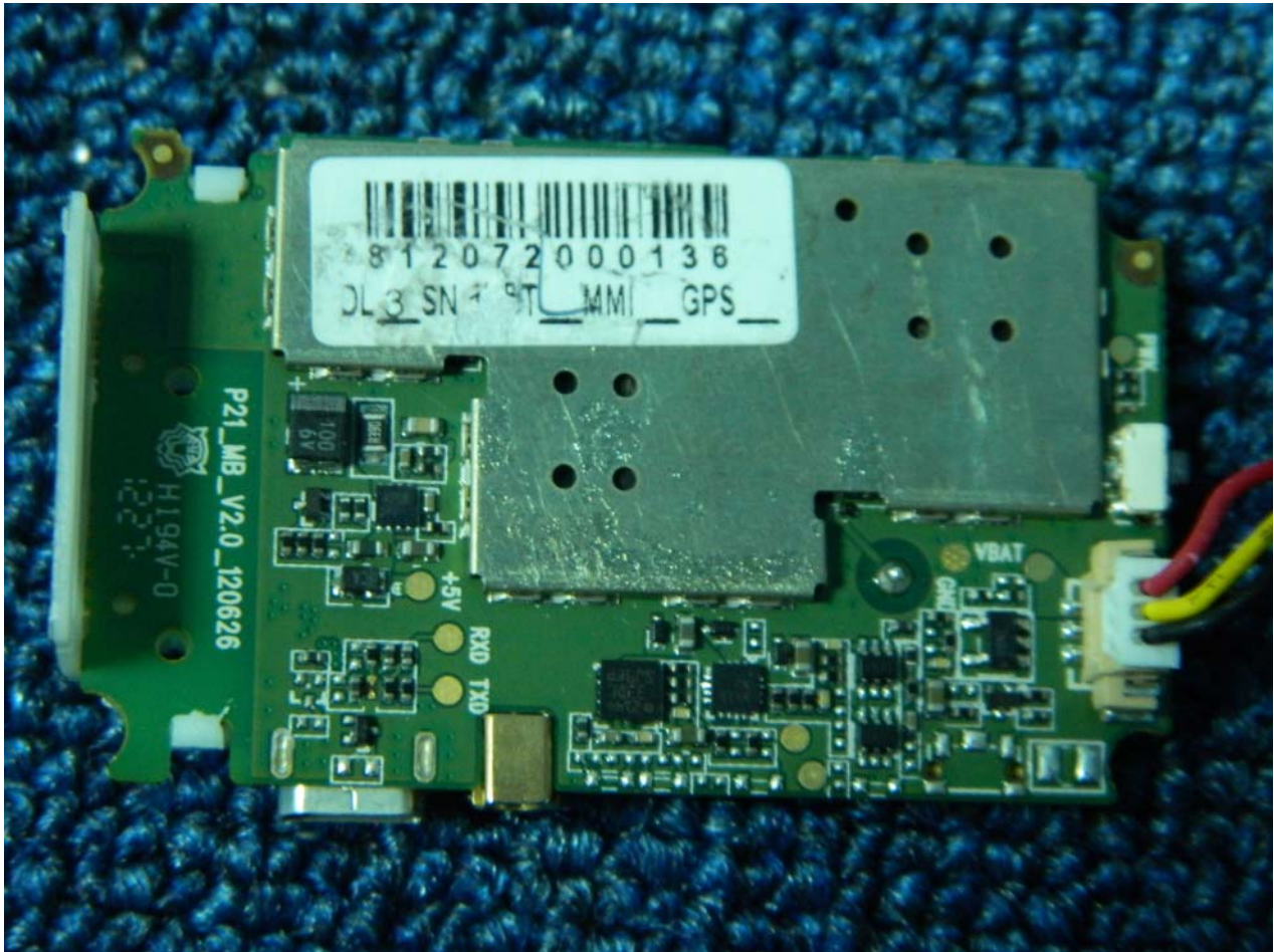
Fig.5 Mainboard (reverse)
