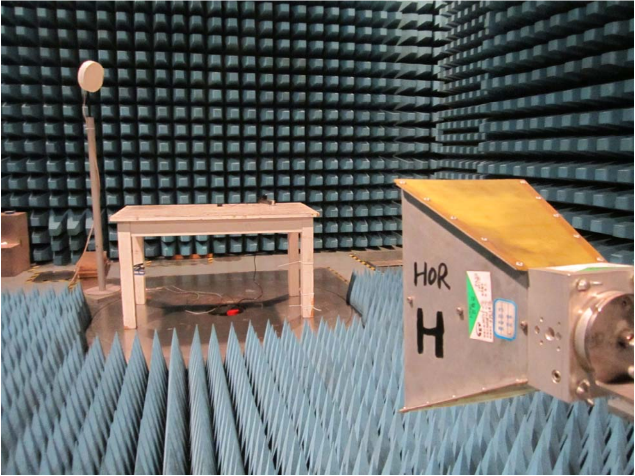
Fig. 3 Radiated emission (1GHz-18GHz) test configuration
