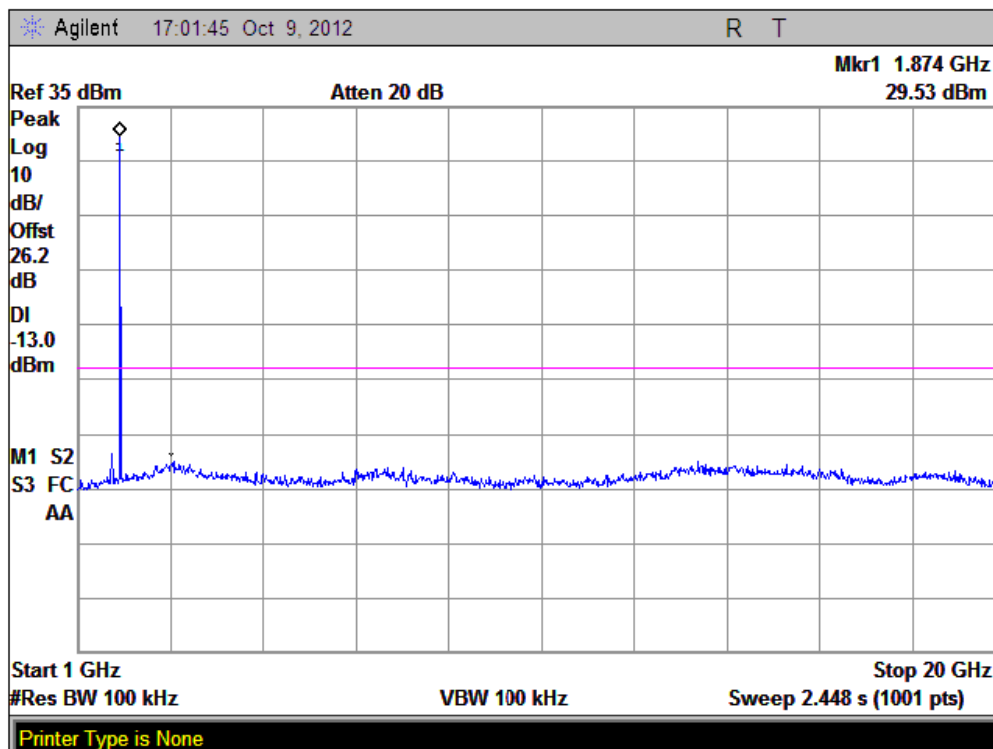
(Plot D2.1: GPRS 1900MHz Channel = 661, 1GHz to 20GHz)
