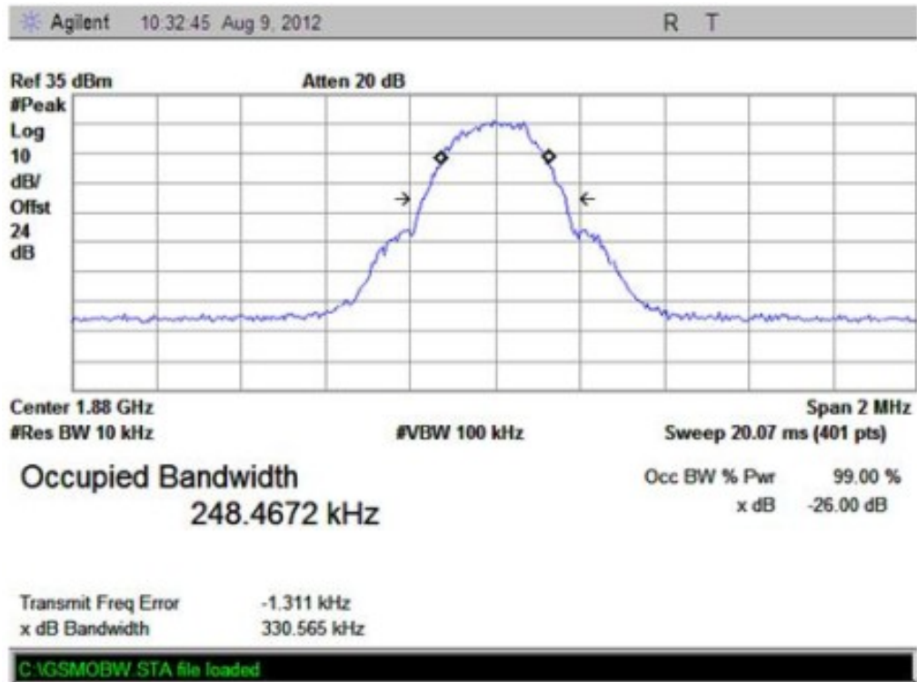
(Plot 5: GSM 1900MHz Channel = 661)
