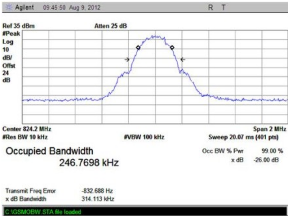
(Plot 1: GSM 850MHz Channel = 128)
