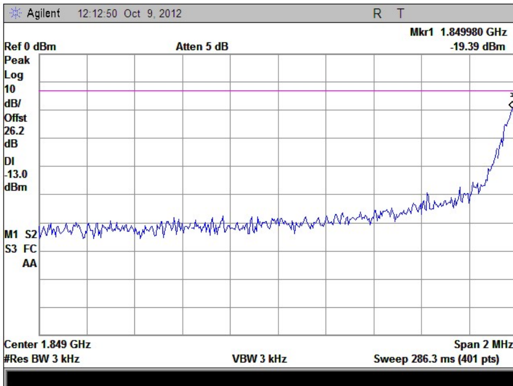
(Plot 7: GPRS 1900 Channel = 512)
