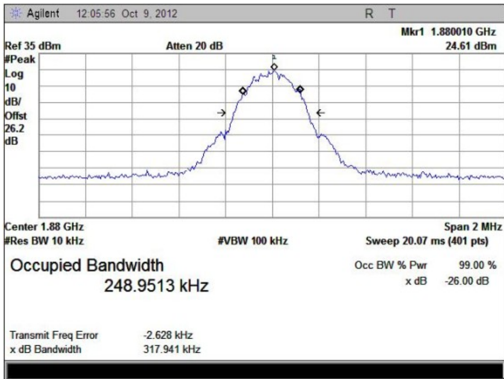
(Plot 11: GPRS 1900MHz Channel = 661)
