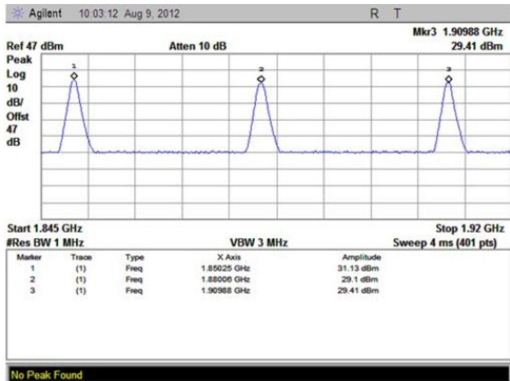
(Plot C: GSM1900MHz Channel = 512, 661, 810)
