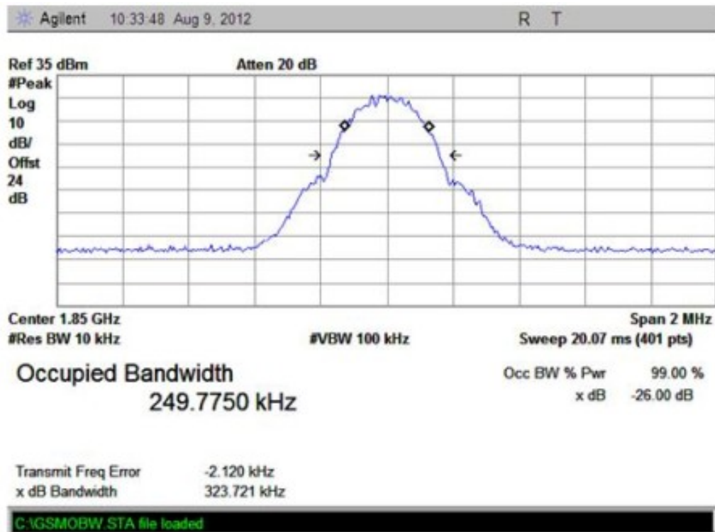
(Plot 4: GSM 1900MHz Channel = 512)
