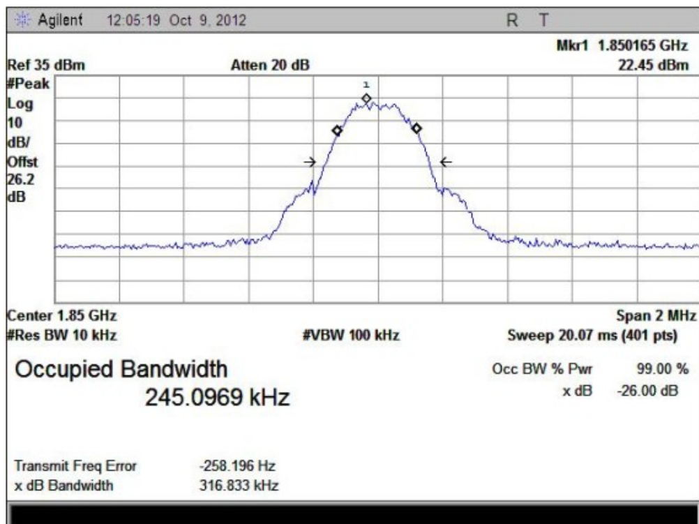
(Plot 10: GPRS 1900MHz Channel = 512)
