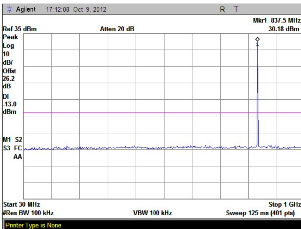
(Plot C2: GPRS 850MHz Channel = 190, 30MHz to 1GHz)
