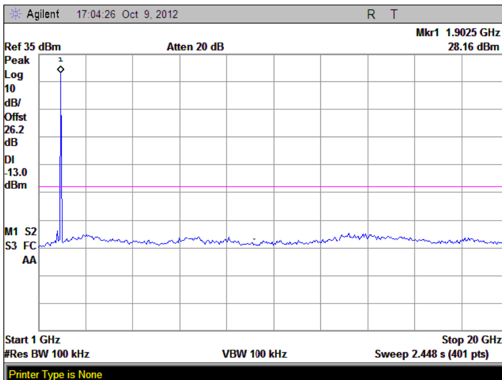
(Plot D3.1: GPRS 1900MHz Channel = 810, 1GHz to 20GHz)
