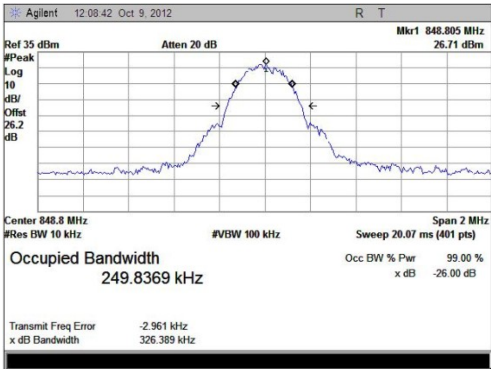
(Plot 9: GPRS 850MHz Channel = 251)
