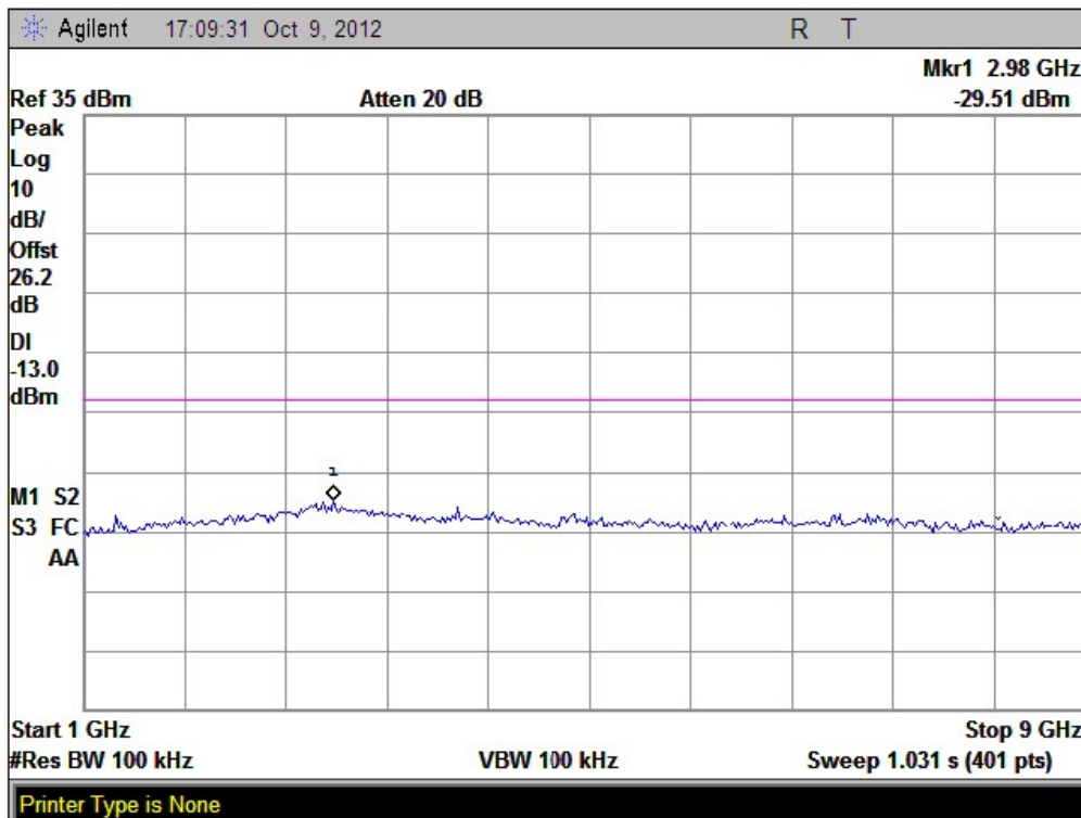
(Plot C1.1: GPRS 850MHz Channel = 128, 1GHz to 9GHz)
