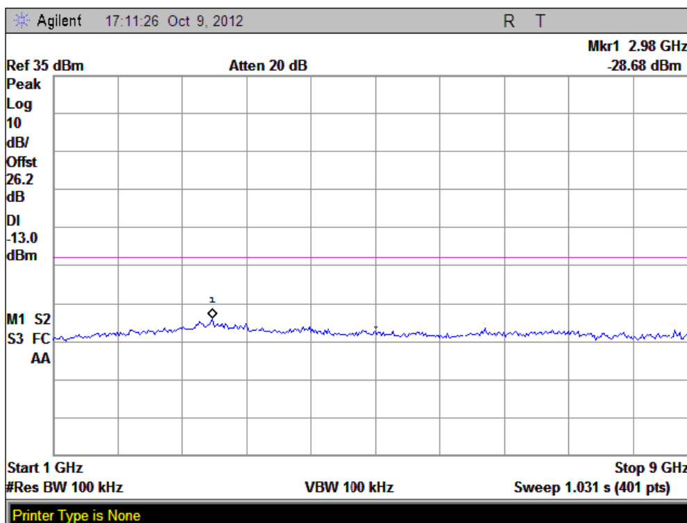
(Plot C2.1: GPRS 850MHz Channel = 190, 1GHz to 9GHz)
