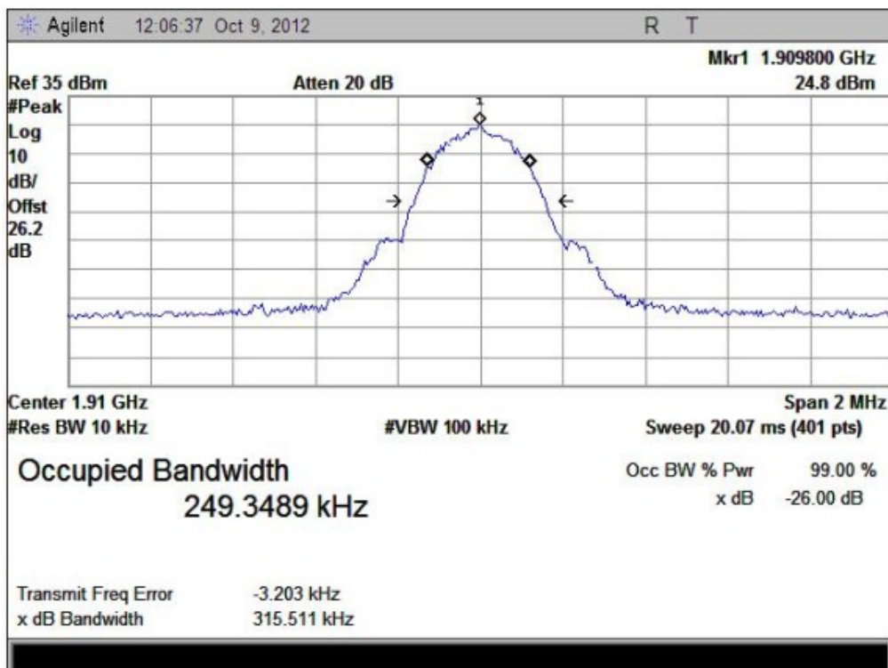
(Plot 12: GPRS 1900MHz Channel = 810)
