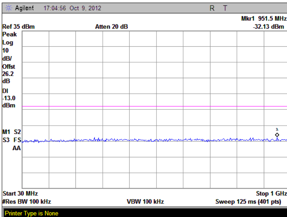
(Plot D3: GPRS 1900MHz Channel = 810, 30MHz to 1GHz)
