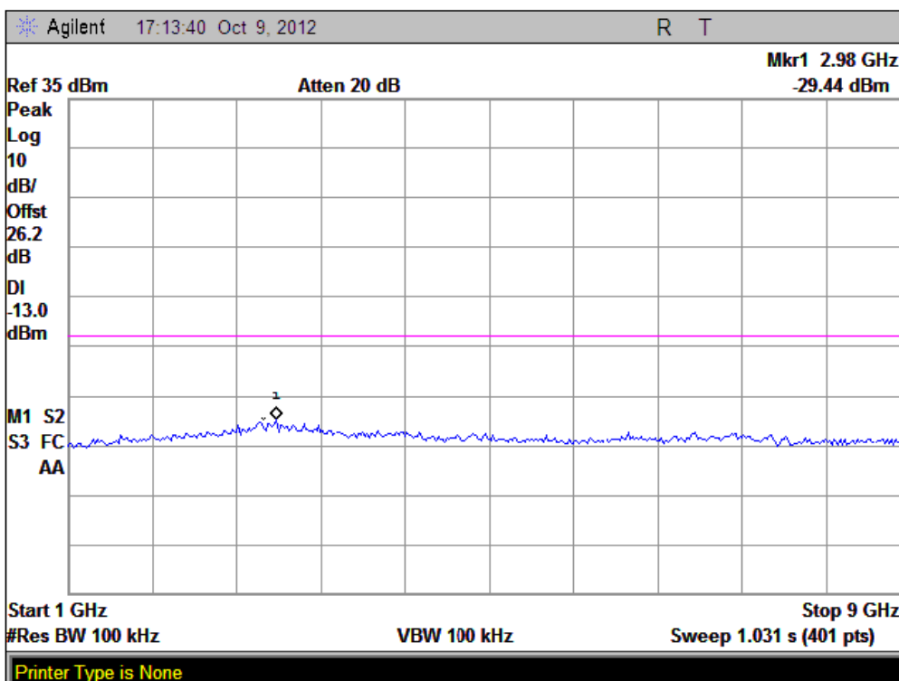
(Plot C3.1: GPRS 850MHz Channel = 251, 1GHz to 9GHz)
