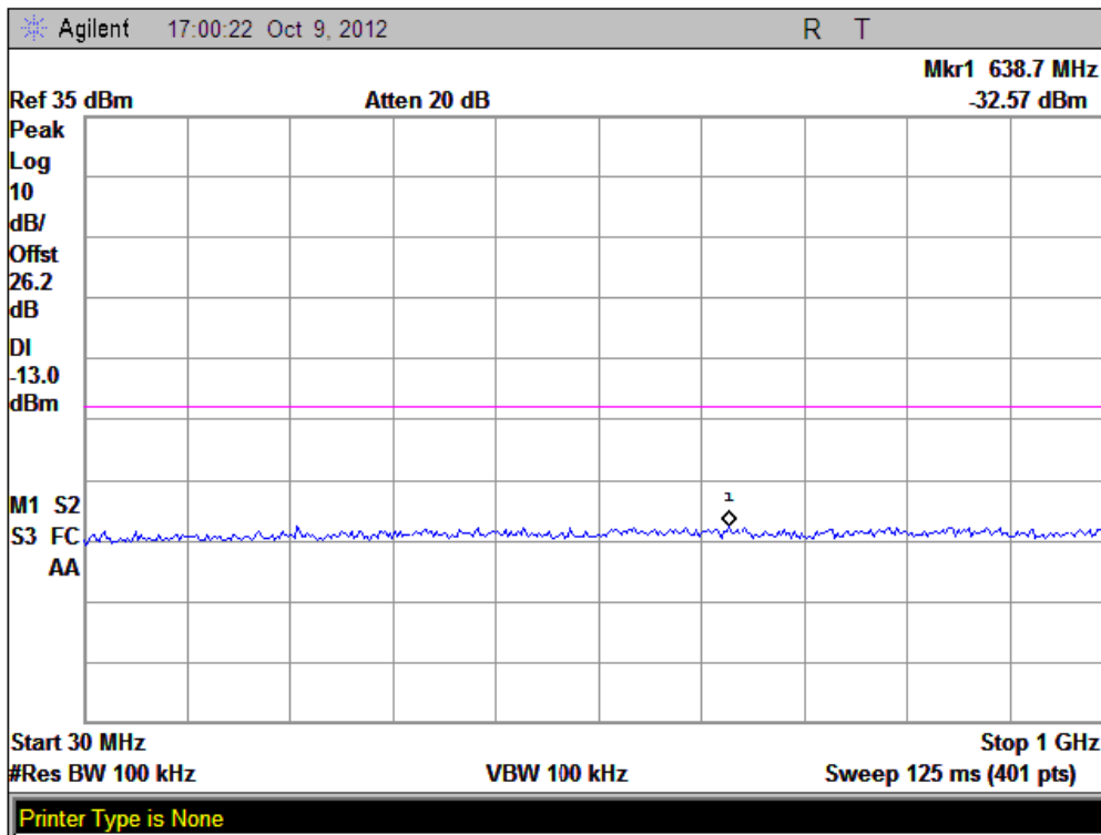
(Plot D2: GPRS 1900MHz Channel = 661, 30MHz to 1GHz)
