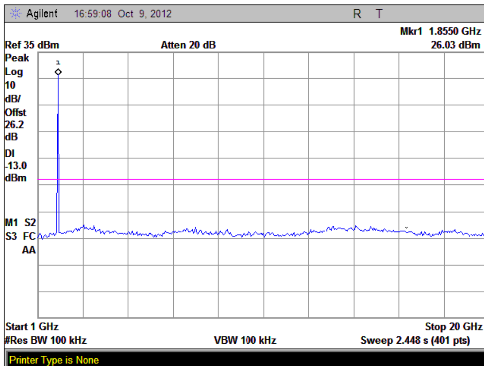
(Plot D1.1: GPRS 1900MHz Channel = 512, 1GHz to 20GHz)
