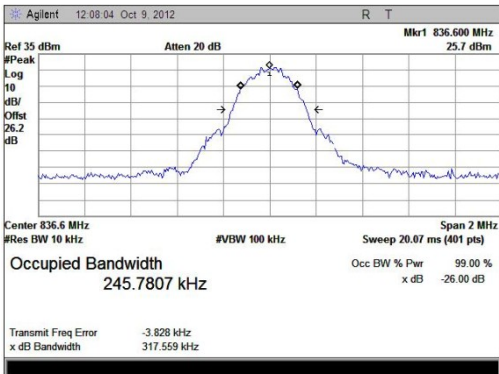
(Plot 8: GPRS 850MHz Channel = 190)
