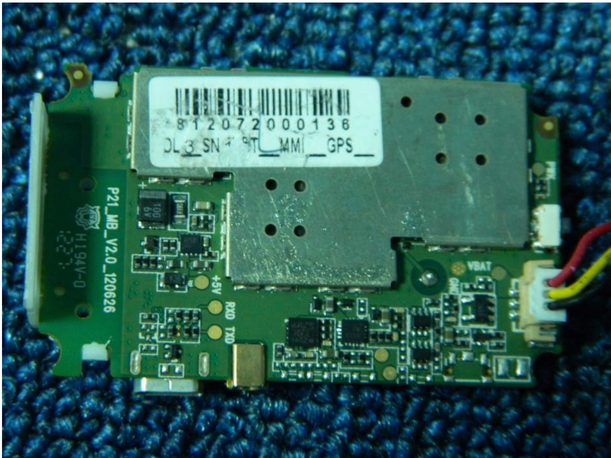
Fig. 3 PCBA (reverse, shielding on)
