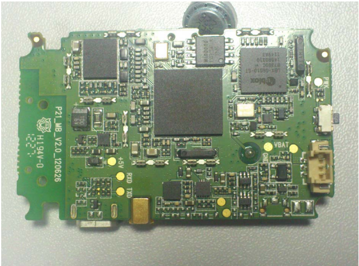
Fig. 4 PCBA (reverse, shielding off)
