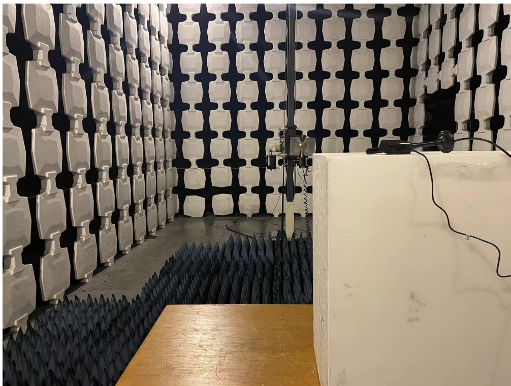
Pic3. Radiated spurious emission (3GHz-18GHz)
