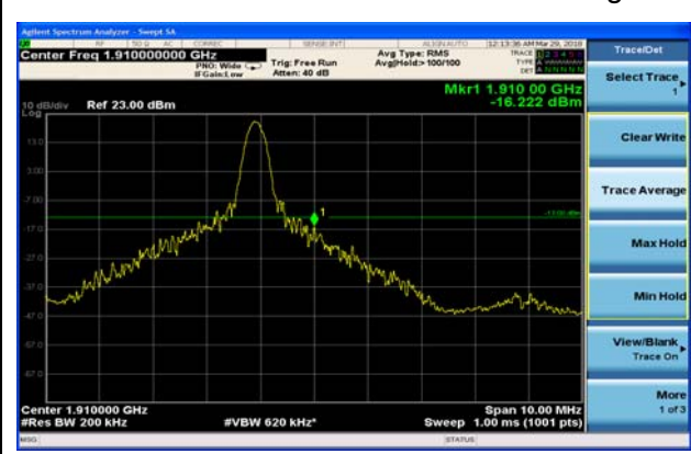
LTE Band 2 20MHz 16QAM 100%RB CH-High
