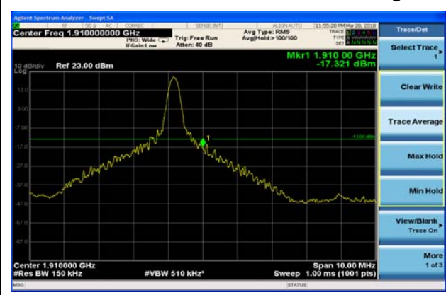
LTE Band 2 15MHz 16QAM 100%RB CH-High
