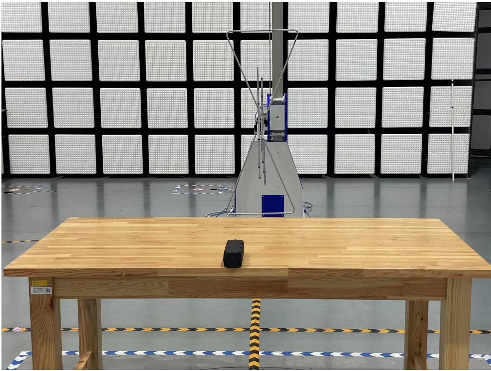
RSE_30MHz-1GHz
