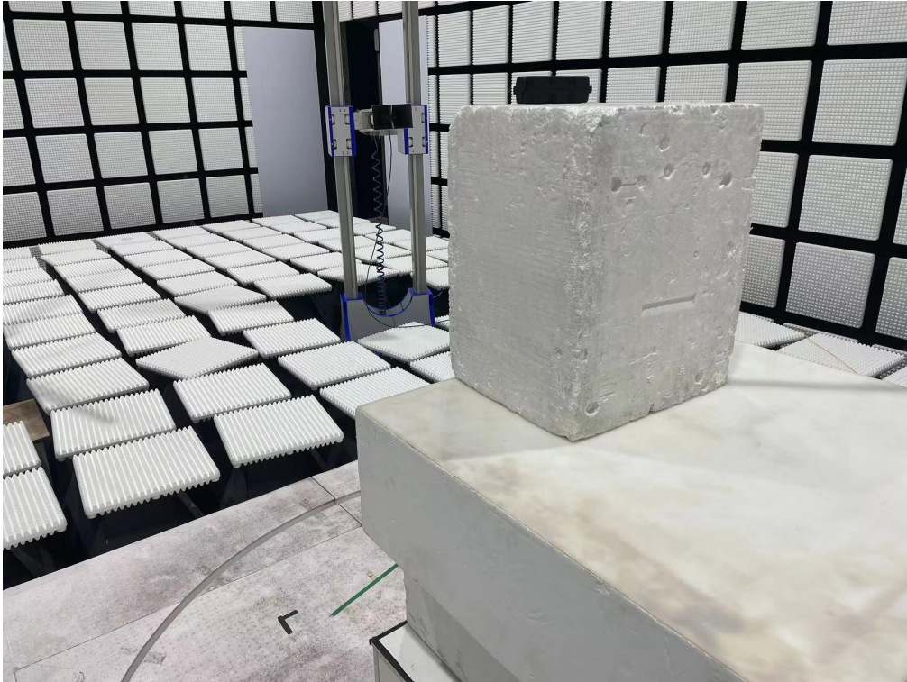
RE 1GHz-5GHz
