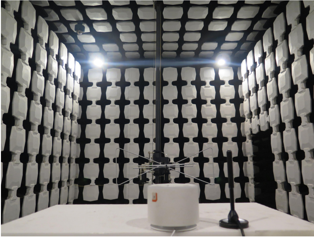
Pic1. Radiated spurious emission (30MHz-1GHz)
