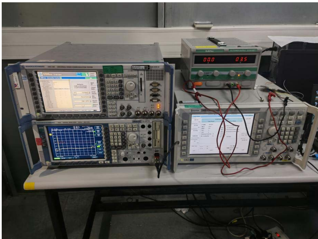
RF test setup photos-WWAN
