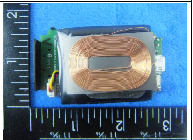
Coil - Front View (only for Wireless Charging)
