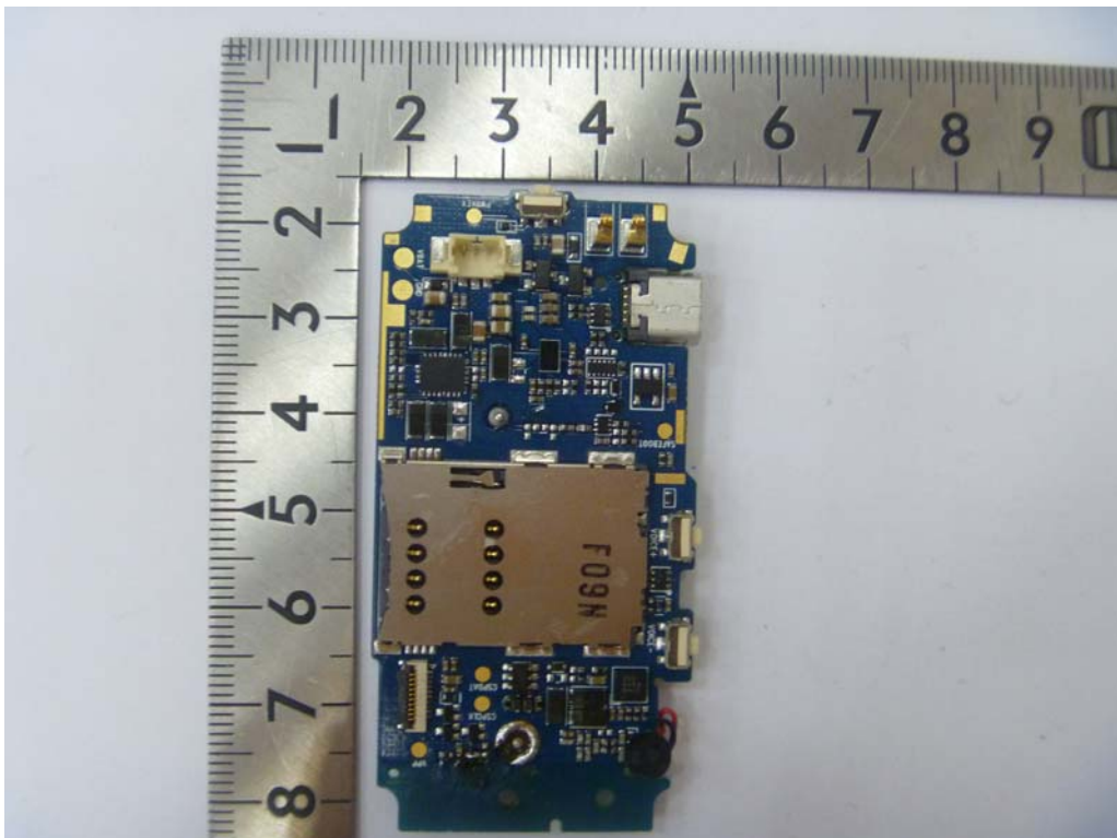
VL2000_Bottom View-2
