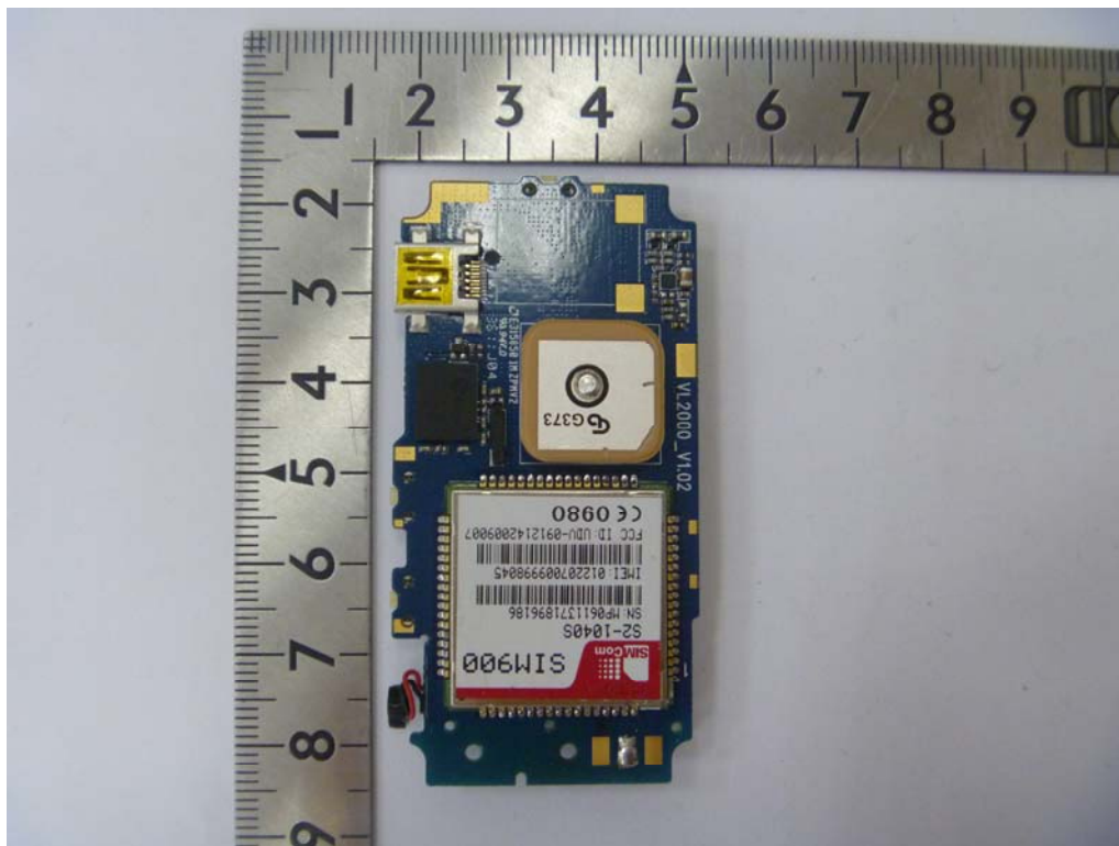
VL2000_Top View-2
