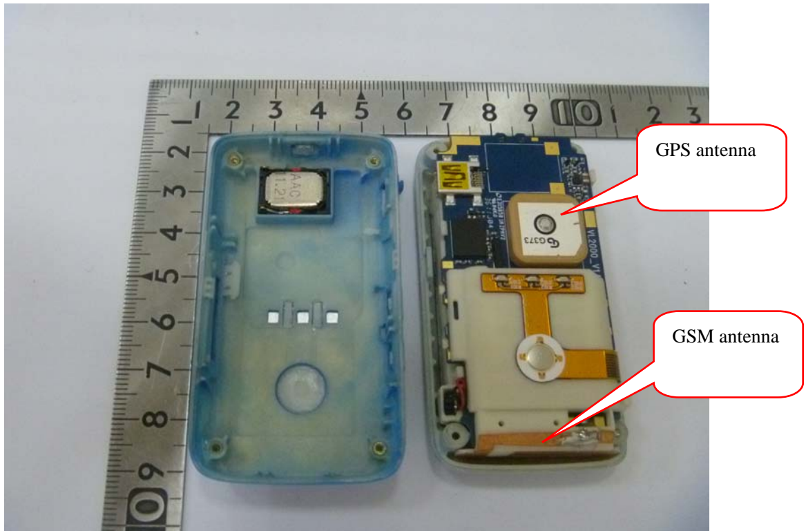
VL2000_Top View-1
