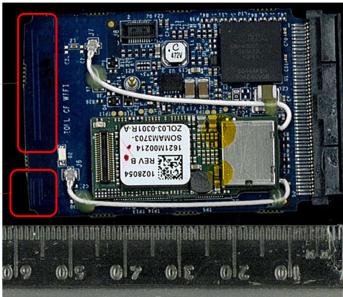
Internal Photos – Zoll CF WIFI Card Top (With SOM)
