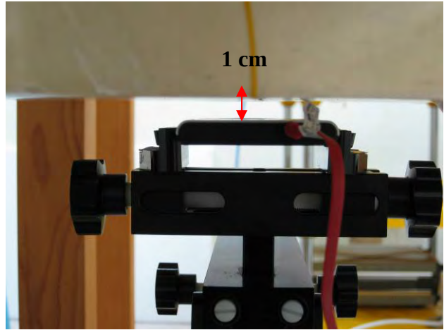
Fig.3 Body worn- EUT rear to flat phantom and distance between flat phantom and mobile phone is 1 cm.
