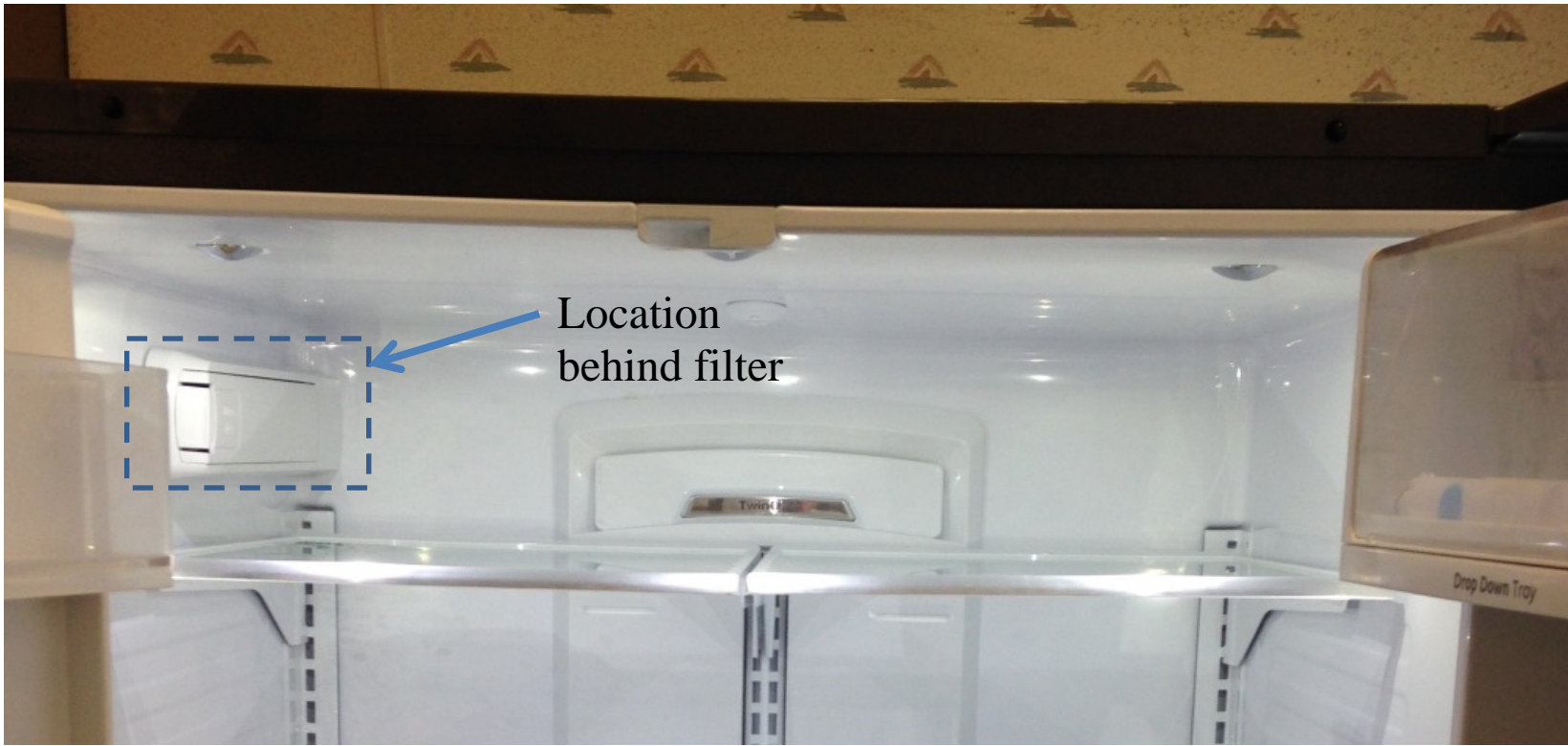
Refrigerator doors open showing water filter location. The RFID board is mounted behind the water filter.
