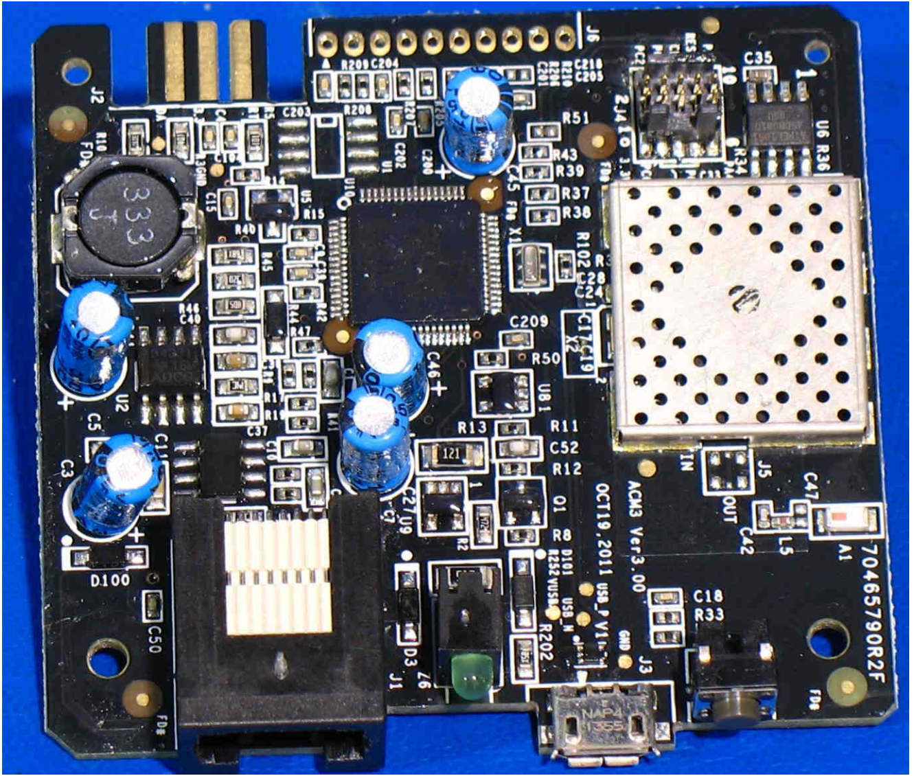
Component Side
