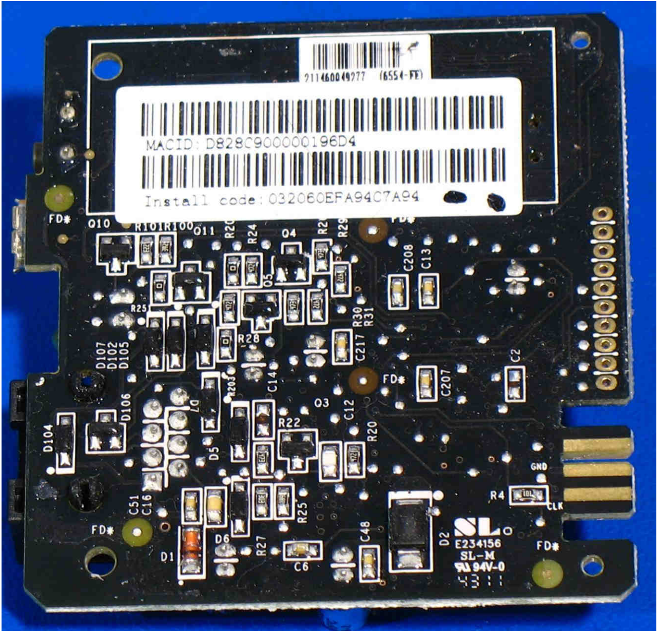
Solder Side
