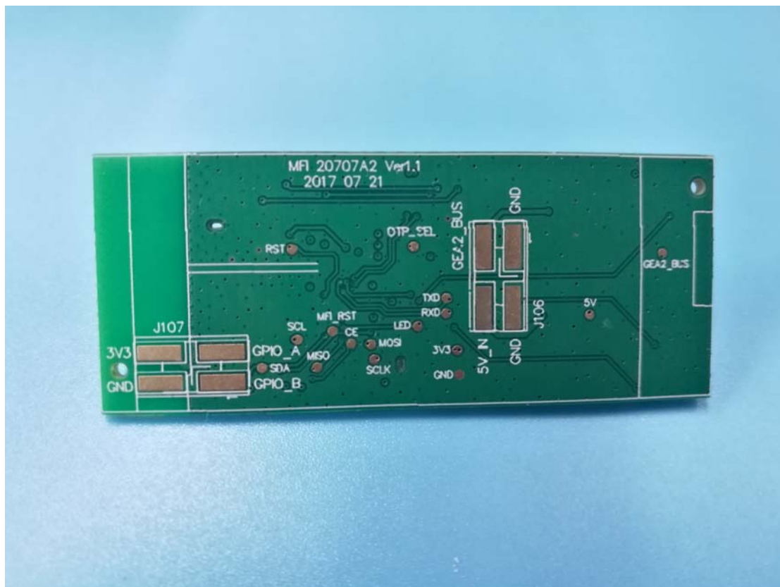
2. Mainboard rear view
