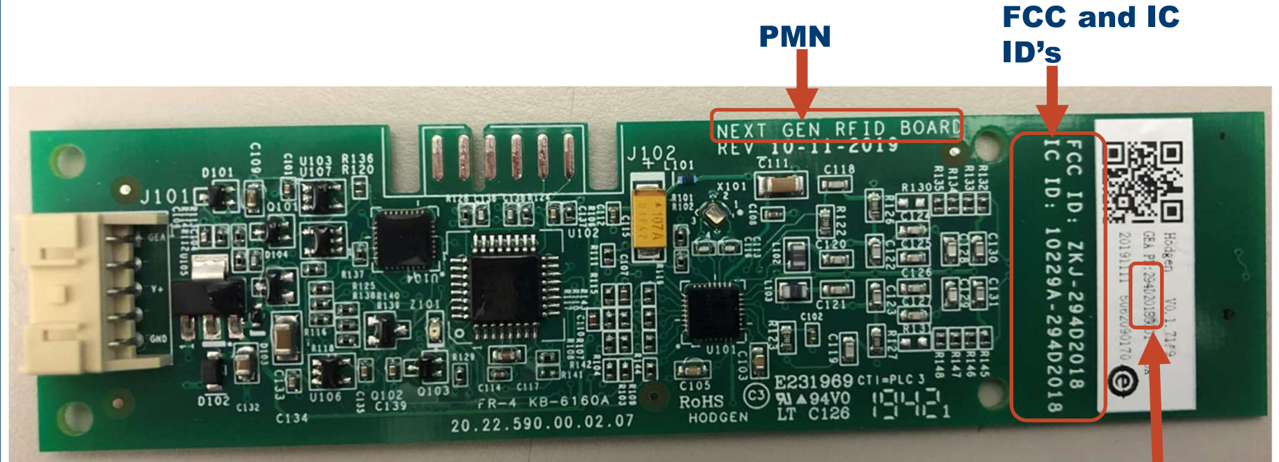
Top Of Board (Detailed locations)
