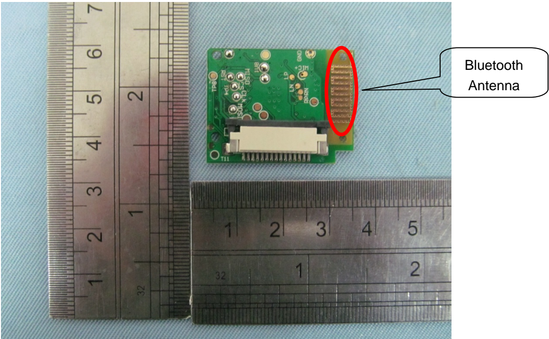
FRONT VIEW OF PCB-1
