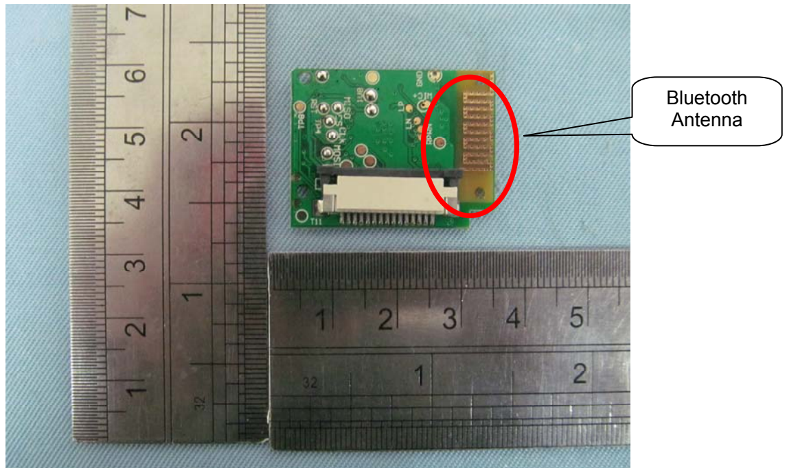
BACK VIEW OF PCB-1
