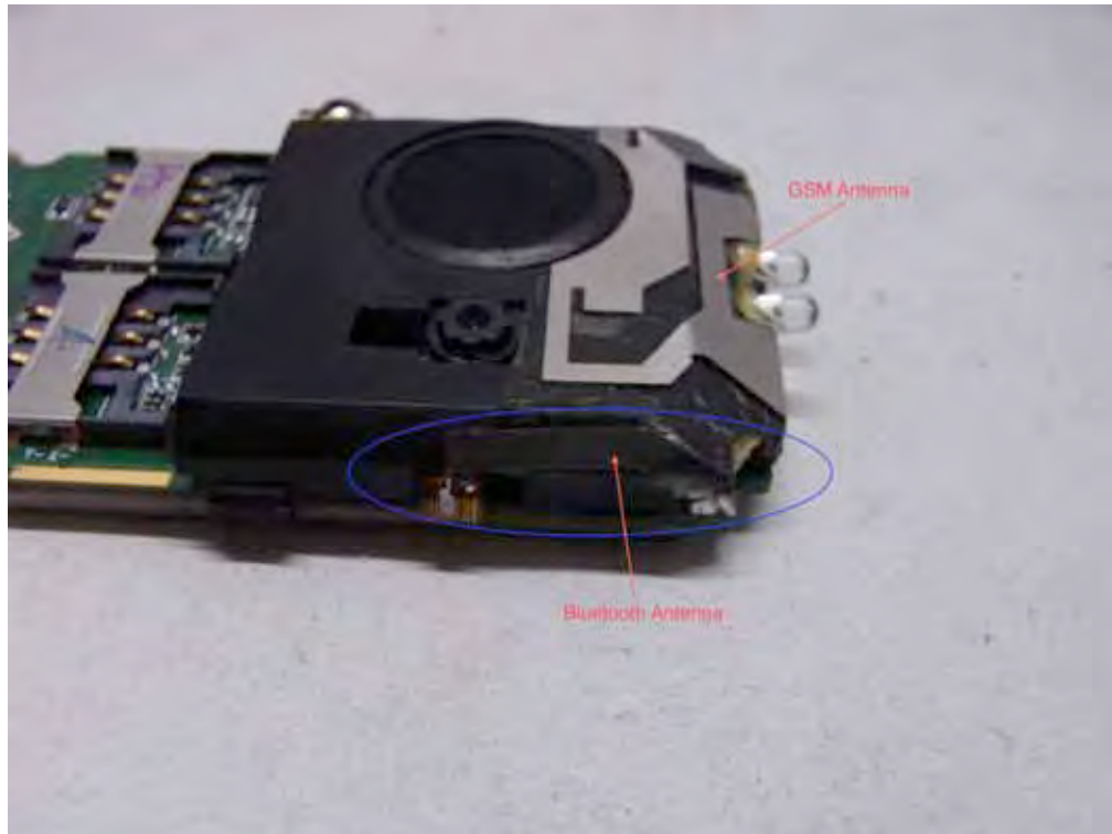
Antenna Photo
