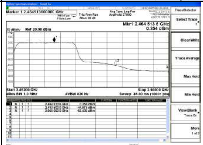
802.11n-HT20 Chain 0-High channel(Average)
