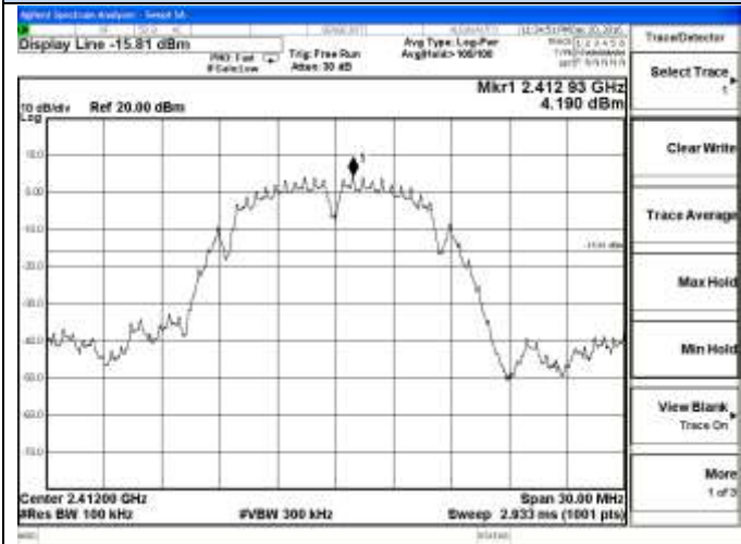
802.11b Chain 1-Low channel Reference
