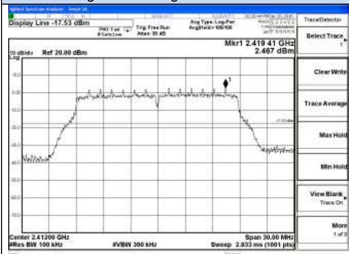
802.11n-HT20 Chain 0-Low channel Reference
