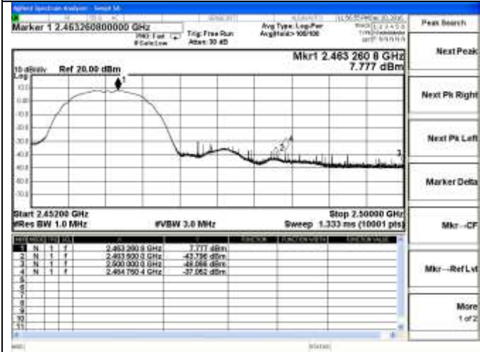
802.11b Chain 1-High channel(Peak)
