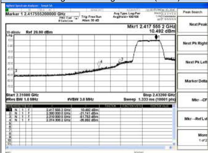
802.11n-HT20 Chain 0-Low channel(Peak)
