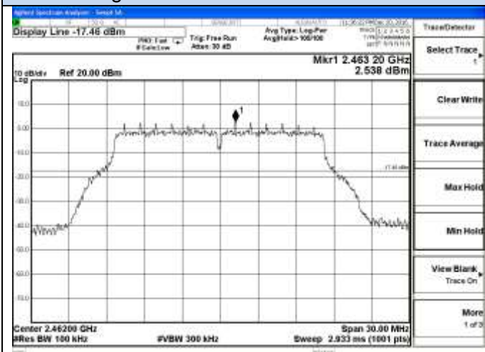
802.11g Chain 1-High channel Reference
