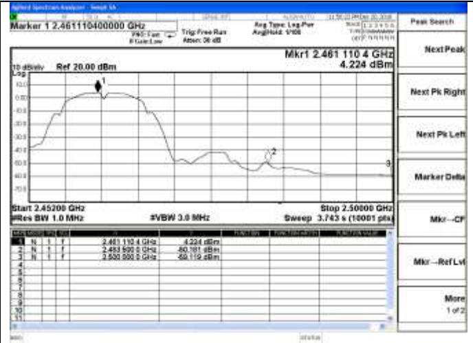
802.11b Chain 1-High channel(Average)
