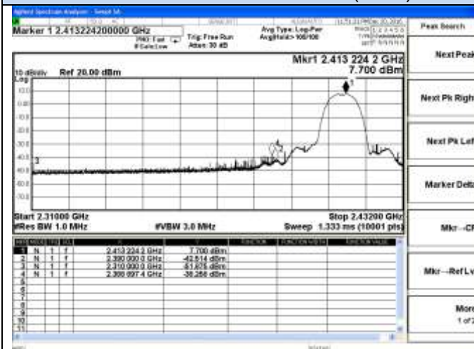
802.11b Chain 1-Low channel(Peak)
