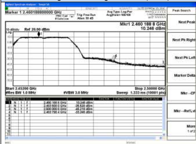
802.11g Chain 1-High channel(Peak)
