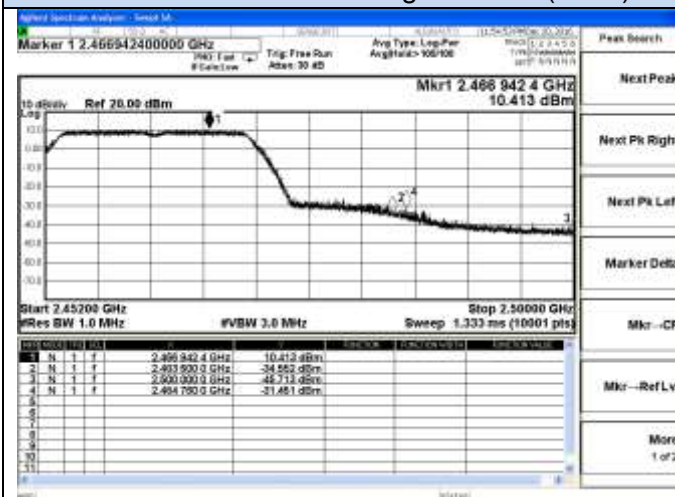
802.11n-HT20 Chain 1-High channel(Peak)
