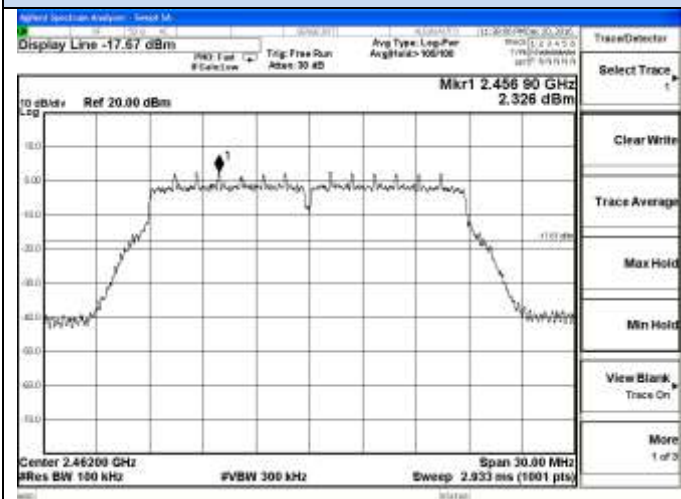
802.11n-HT20 Chain 1-High channel Reference
