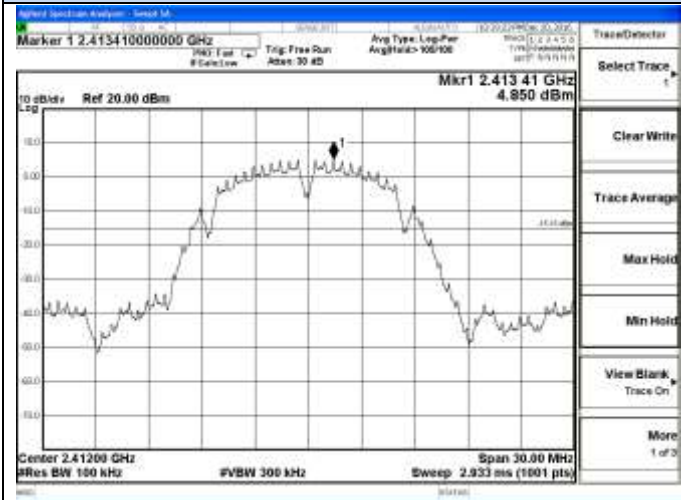
802.11b Chain 0-Low channel Reference
