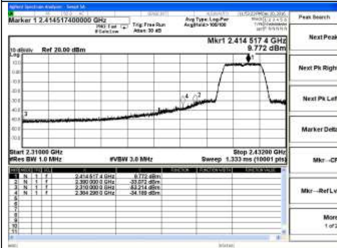
802.11n-HT20 Chain 1-Low channel(Peak)
