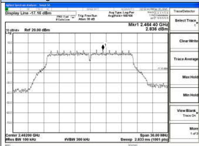
802.11g Chain 0-High channel Reference
