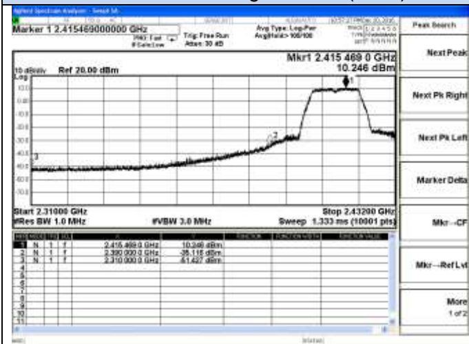
802.11g Chain 0-Low channel(Peak)
