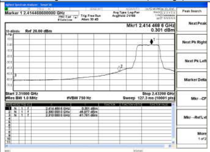
802.11g Chain 1-Low channel(Average)
