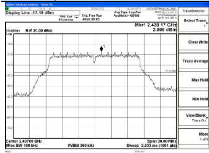
802.11g Chain 0-Middle channel Reference
