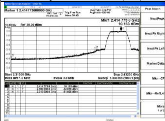
802.11g Chain 1-Low channel(Peak)
