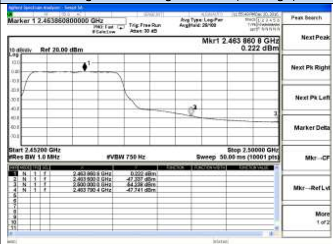
802.11g Chain 1-High channel(Average)
