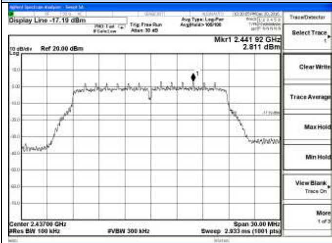
802.11n-HT20 Chain 0-Middle channel Reference
