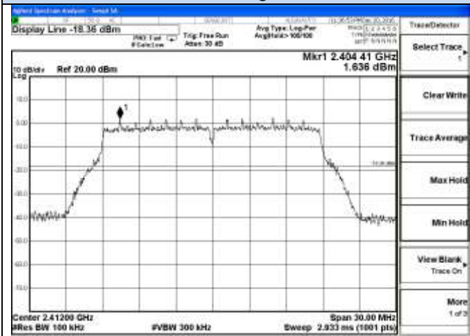
802.11n-HT20 Chain 1-Low channel Reference
