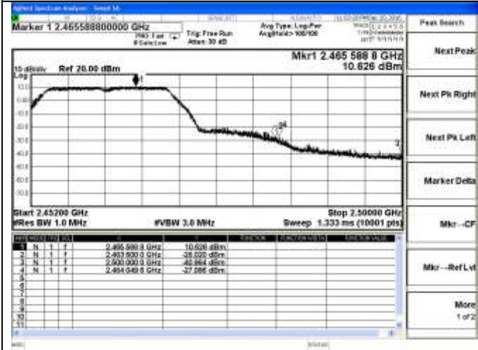
802.11g Chain 0-High channel(Peak)
