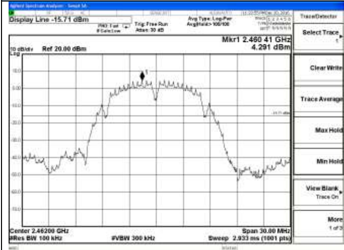
802.11b Chain 1-High channel Reference
