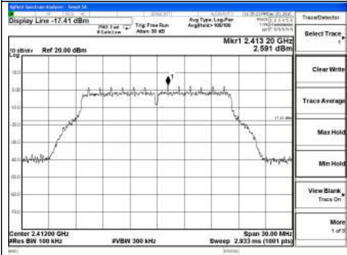
802.11g Chain 1-Low channel Reference
