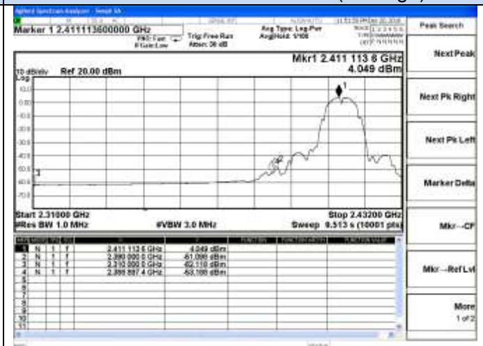
802.11b Chain 1-Low channel(Average)
