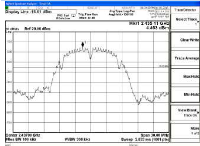
802.11b Chain 1-Middle channel Reference
