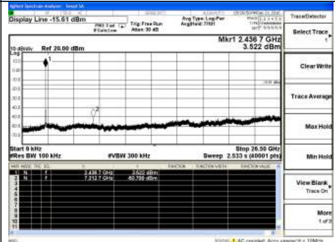
802.11b Chain 1-Middle channel
