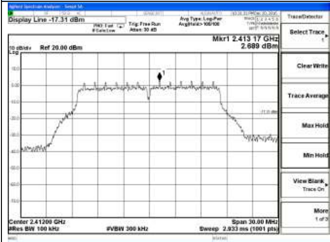
802.11g Chain 0-Low channel Reference
