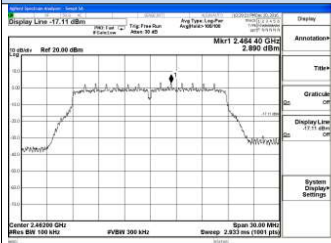
802.11n-HT20 Chain 0-High channel Reference
