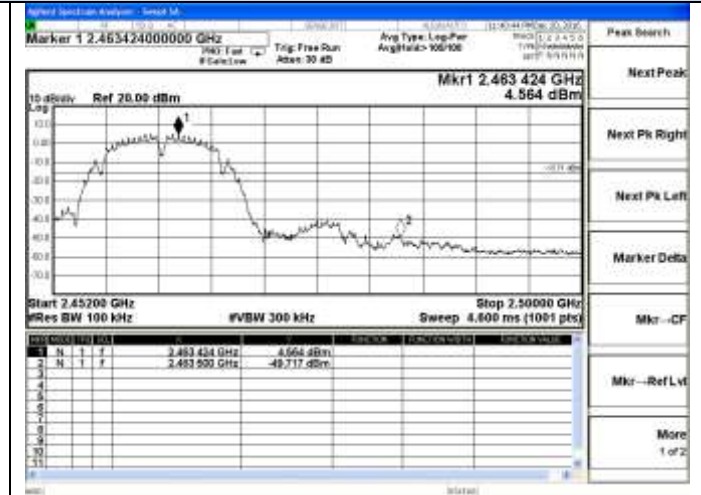
802.11b Chain 1-High channel
