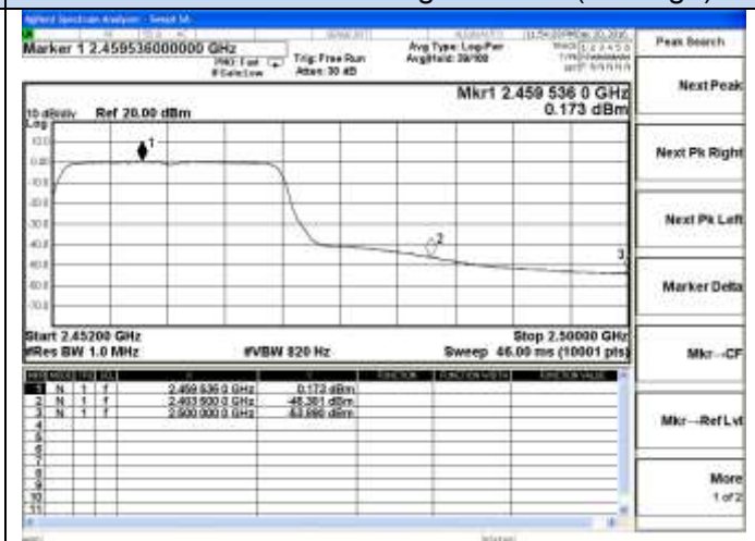
802.11n-HT20 Chain 1-High channel(Average)
