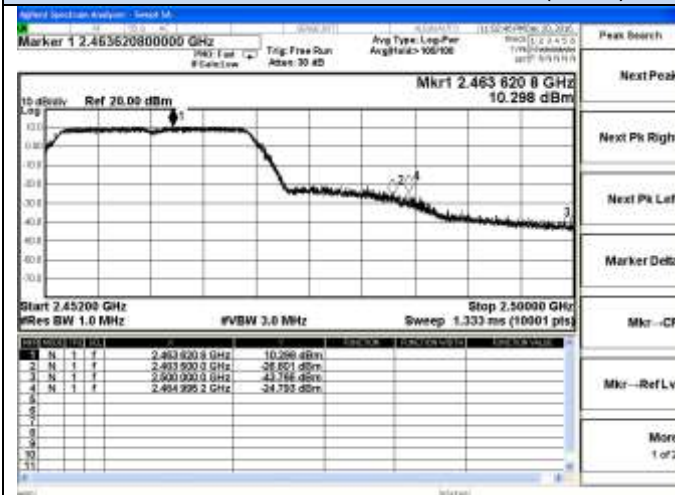
802.11n-HT20 Chain 0-High channel(Peak)
