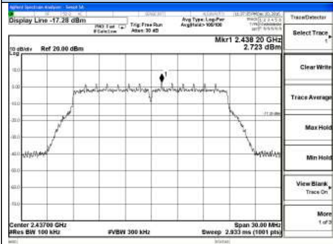
802.11n-HT20 Chain 1-Middle channel Reference
