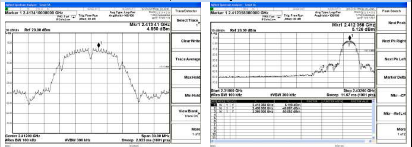
802.11b Chain 0-Low channel Reference
