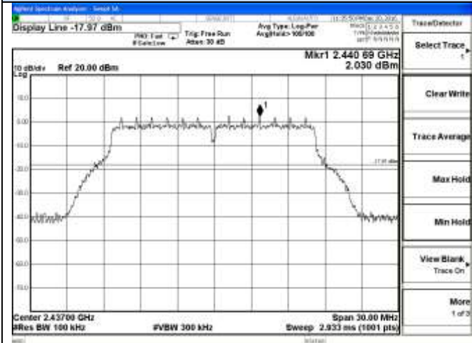
802.11g Chain 1-Middle channel Reference
