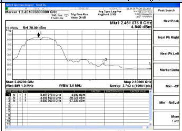
802.11b Chain 0-High channel(Average)
