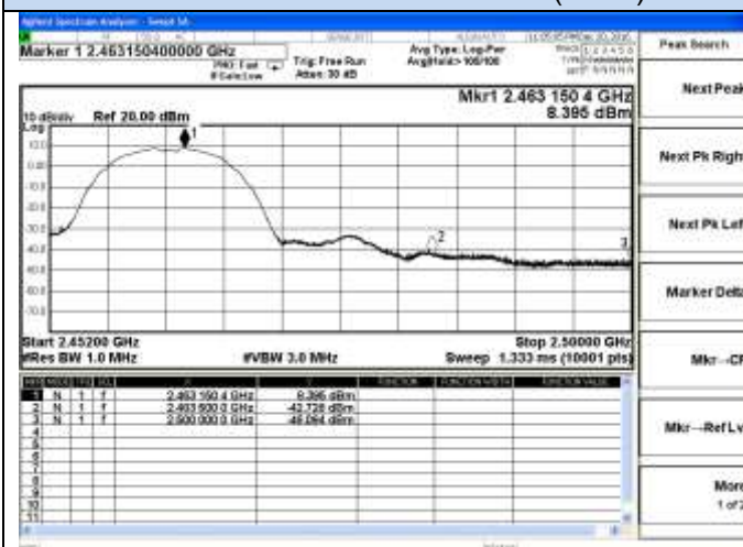
802.11b Chain 0-High channel(Peak)
