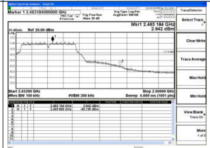
802.11g Chain 0-High channel
