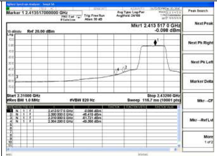
802.11n-HT20 Chain 1-Low channel(Average)
