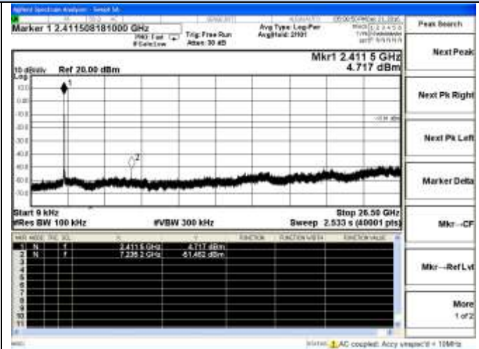
802.11b Chain 1-Low channel
