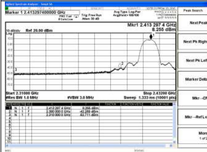
802.11b Chain 0-Low channel(Peak)
