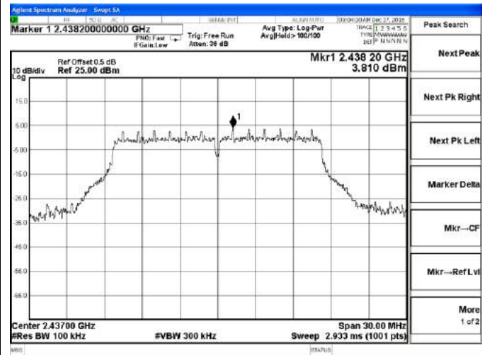
Channel 6 / 2437 MHz
