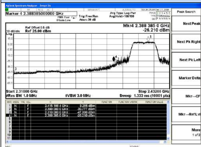
Channel 1 / 2412 MHz – Peak
