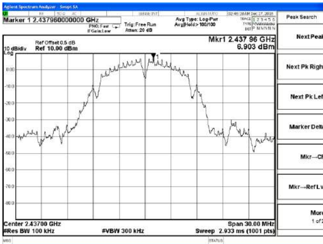
Channel 6 / 2437 MHz
