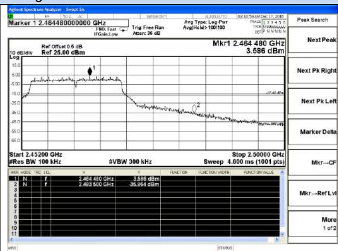
Channel 11 / 2462 MHz
