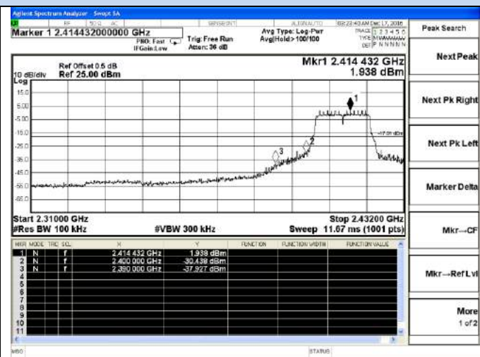
Channel 1 / 2412 MHz
