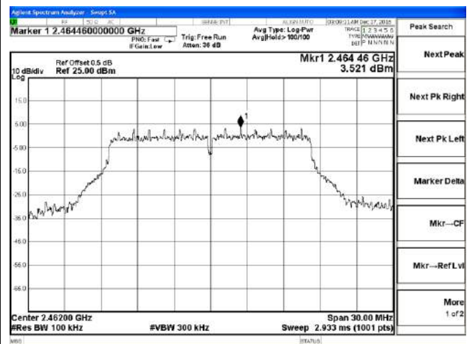
Channel 11 / 2462 MHz
