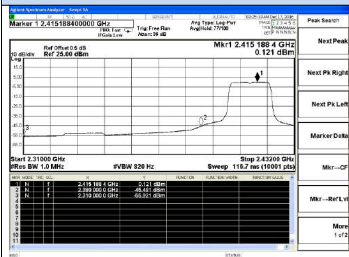
Channel 1 / 2412 MHz – Average
