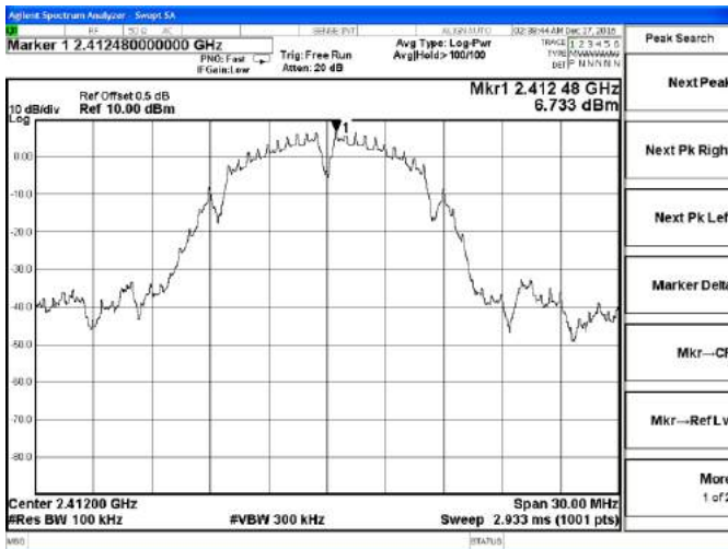
Channel 1 / 2412 MHz
