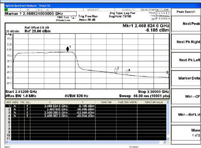
Channel 11 / 2462 MHz – Average
