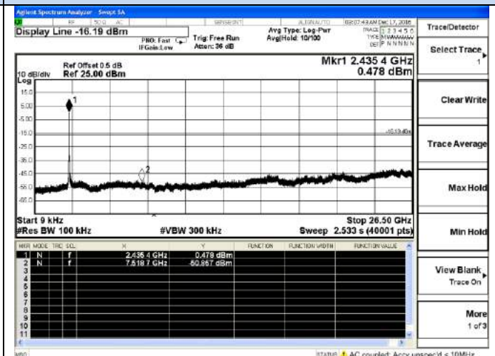
9 KHz – 26.5 GHz
