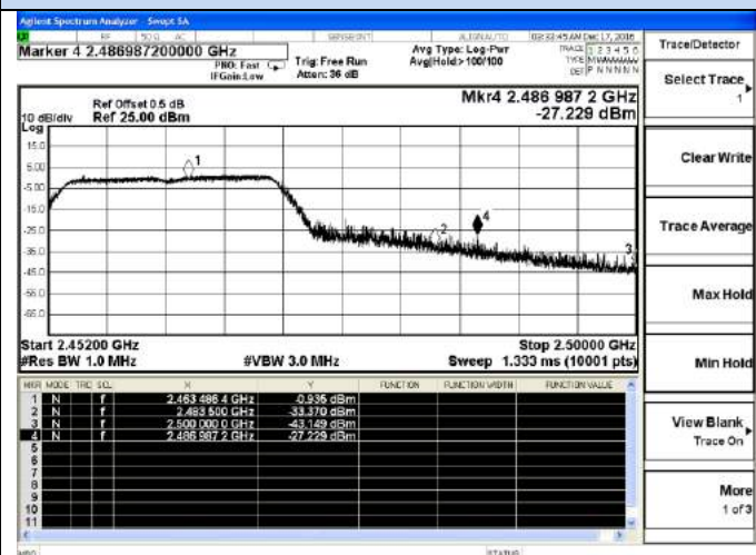
Channel 11 / 2462 MHz – Peak
