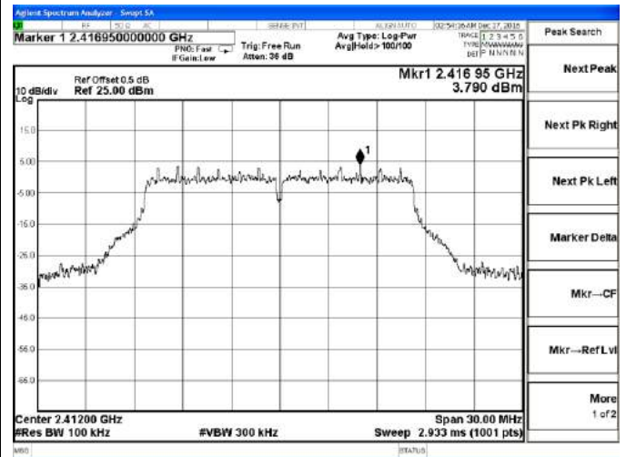
Channel 1 / 2412 MHz
