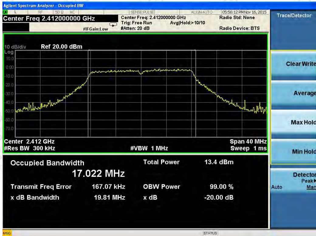
802.11g channel, 20dB bandwidth
