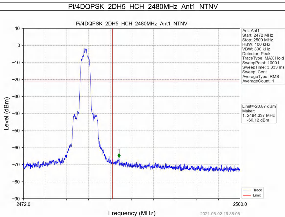
Pi/4DQPSK_2DH5_HCH_2480MHz_Ant1_NTNV
