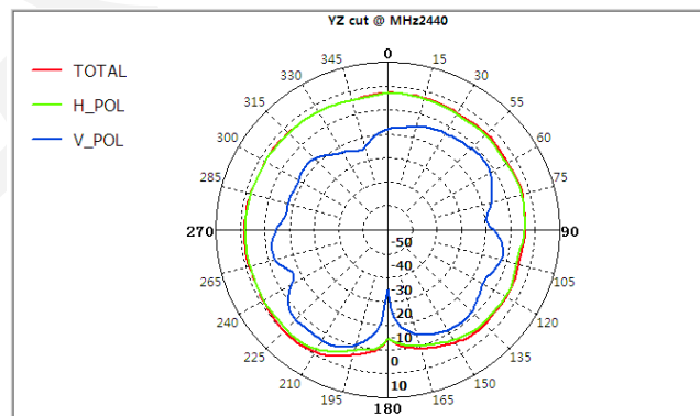
2D-plane YOZ @2.44GHz
