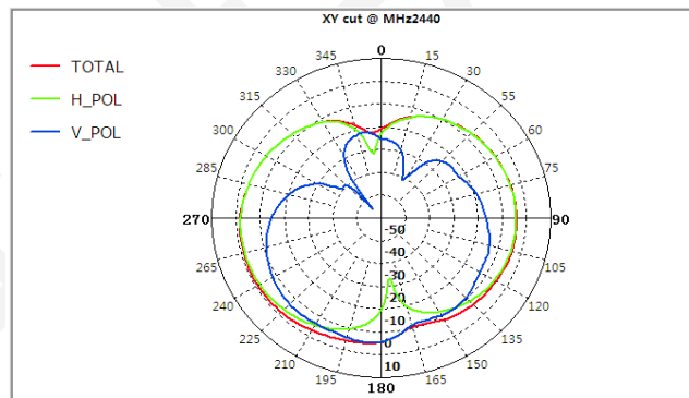
2D-plane XOY @2.44GHz
