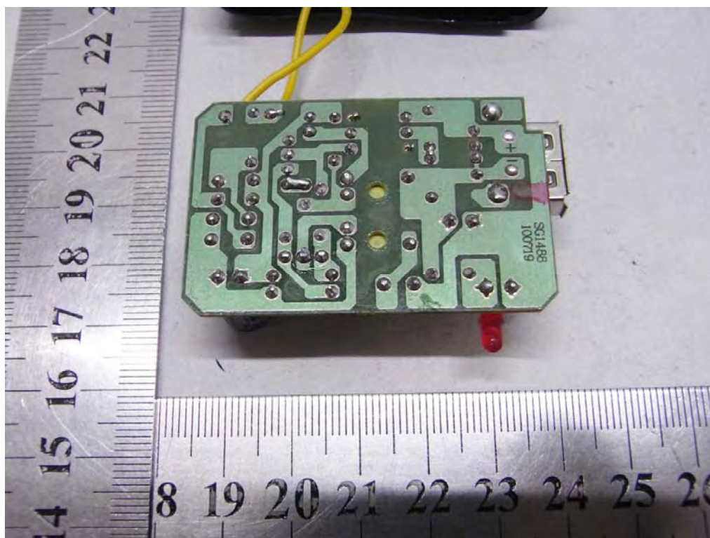
INTERNAL PHOTO OF CHARGER - 2
