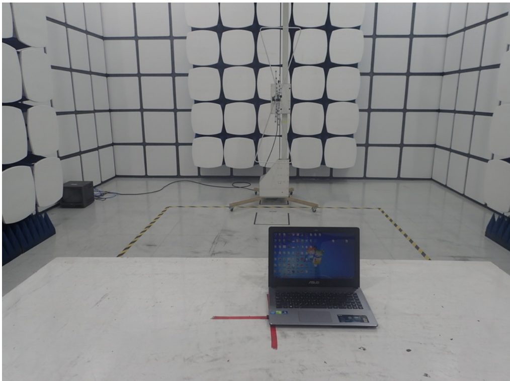
RADIATED EMISSION TEST SETUP BELOW 1GHz
