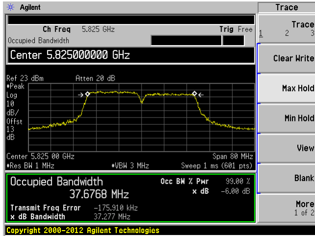
Antenna 1 & 3
