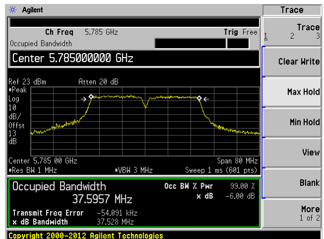
Antenna 2 & 4
