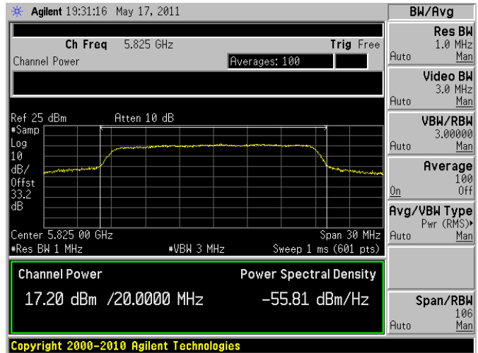
EIRP +36 dBm ~ High Channel
