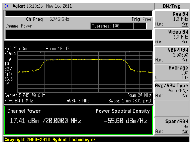
EIRP +36 dBm ~ Low Channel
