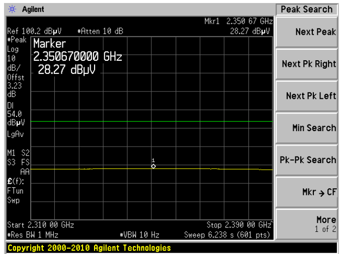
2412 MHz, Lowest Channel at Vertical, Average
