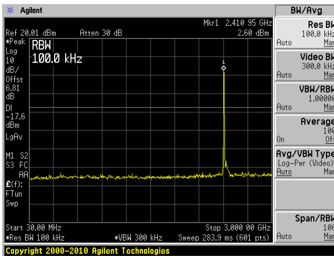
Low Channel
