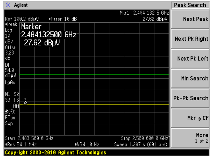
2462 MHz, Highest Channel at Horizontal, Average
