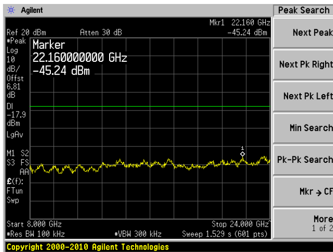
High Channel
