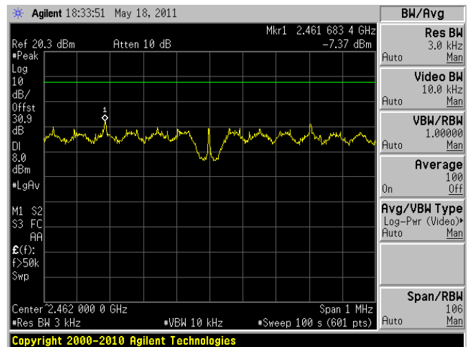
EIRP +30 dBm ~ High Channel
