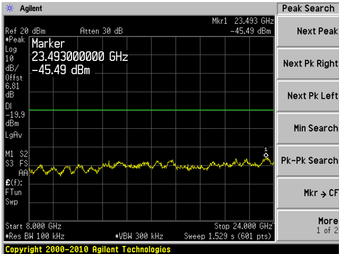
Low Channel
