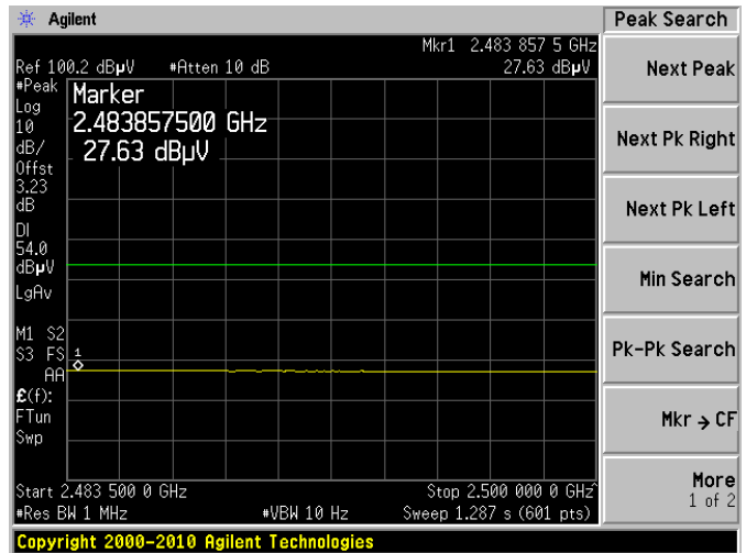
2462 MHz, Highest Channel at Vertical, Average
