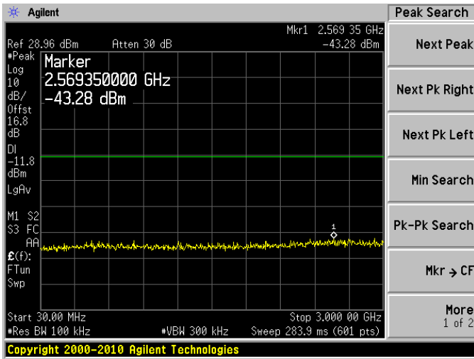
Middle Channel
