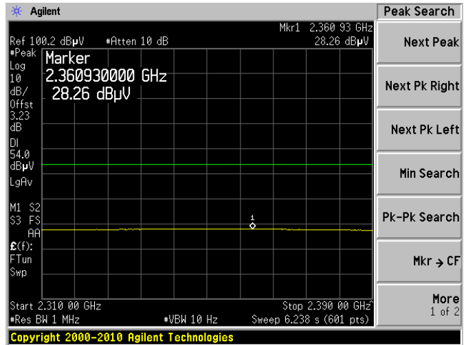
2412 MHz, Lowest Channel at Horizontal, Average
