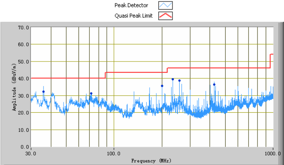
30MHz ~1000MHz Result @ 3m
