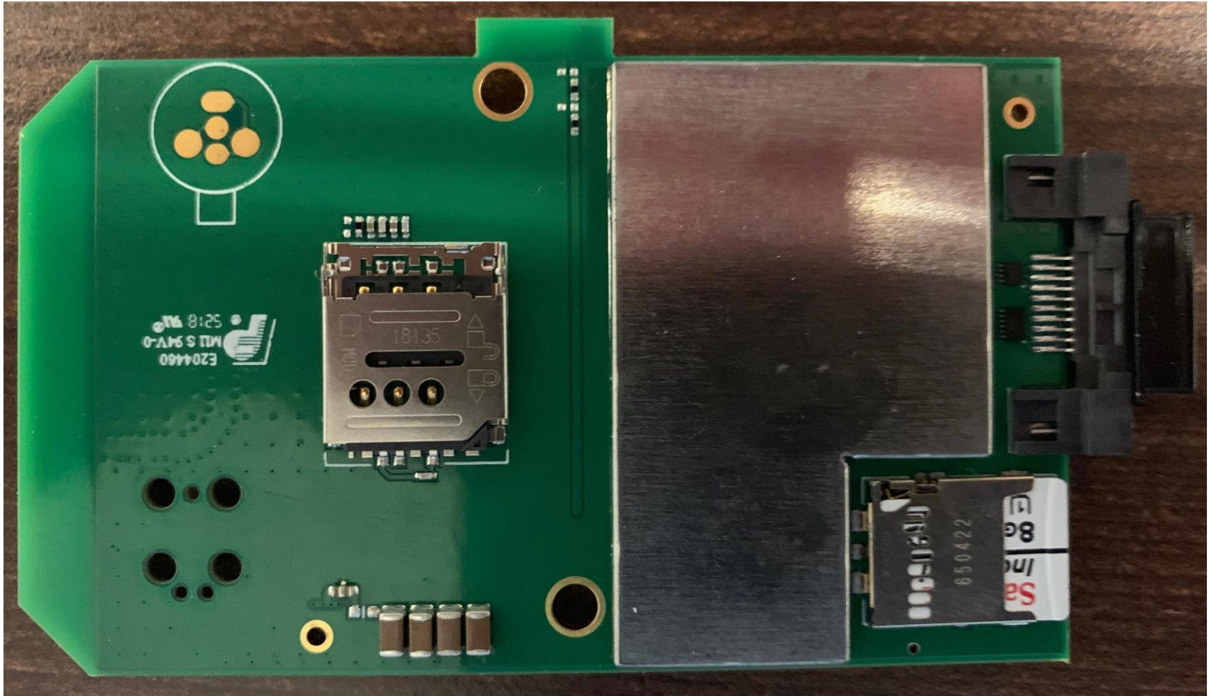
Exhibit: Internal Photos (Bottom PCBA with EMI Shield) (FCC ID: ZIMH40L; EUT IC ID: 9647A-H40L)
