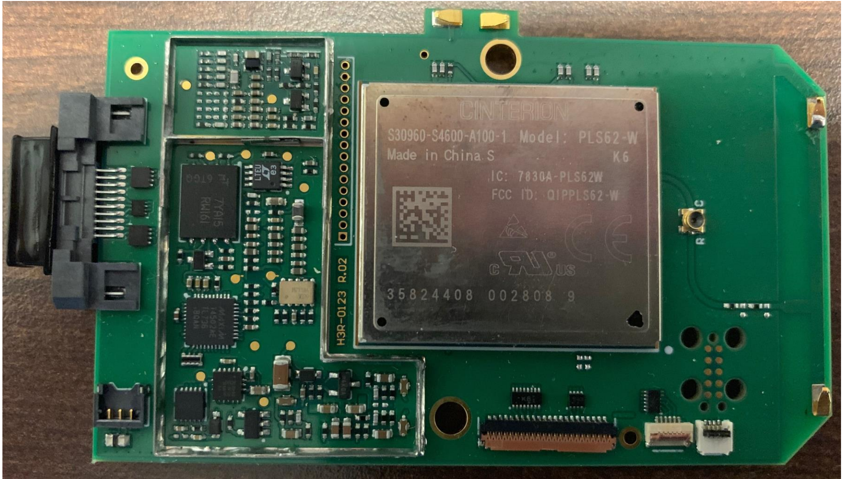
Exhibit: Internal Photos (Top PCBA with EMI Shield Removed) (FCC ID: ZIMH40L; EUT IC ID: 9647A-H40L)
