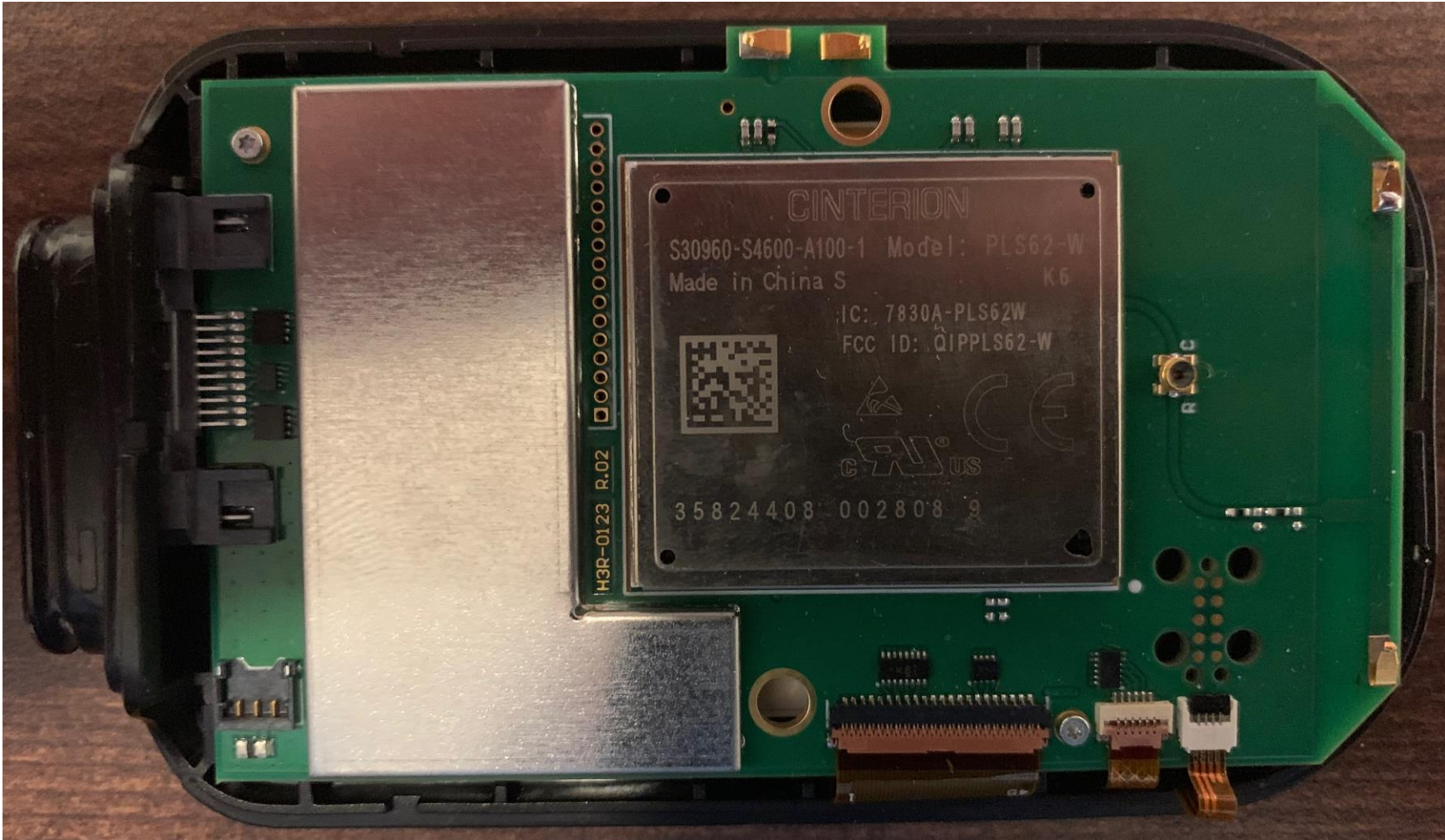
Exhibit: Internal Photos (Interior with Battery Holder / Antenna Removed) (FCC ID: ZIMH40L; EUT IC ID: 9647A-H40L)
