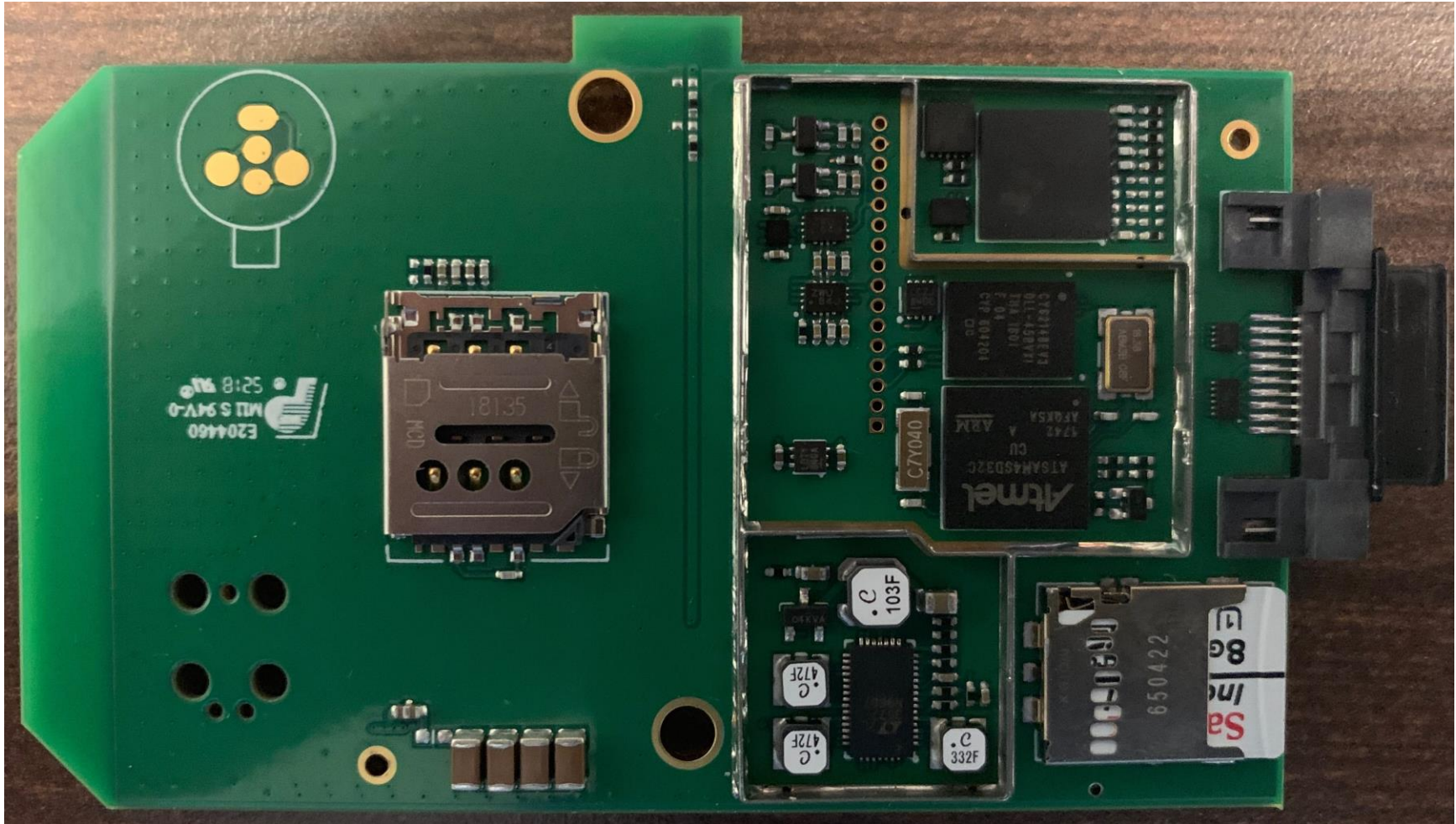
Exhibit: Internal Photos (Bottom PCBA with EMI Shield Removed) (FCC ID: ZIMH40L; EUT IC ID: 9647A-H40L)
