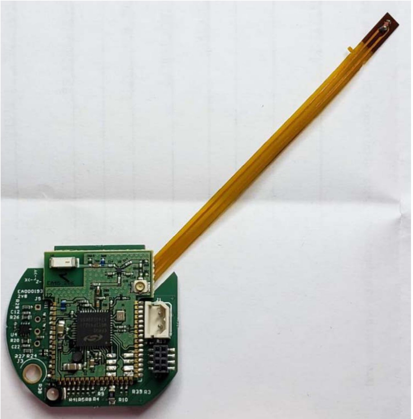
Figure E22A.2 – Internal Photo – Host 1 Internal – PCB Top View
