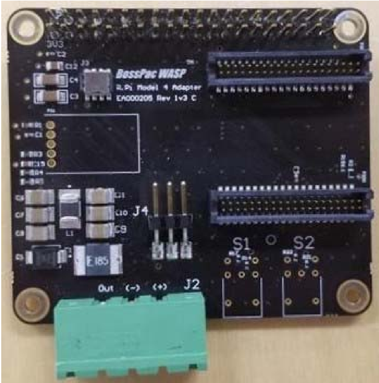
Figure E11B.3 – Internal, EA000406, PCB2 Top
